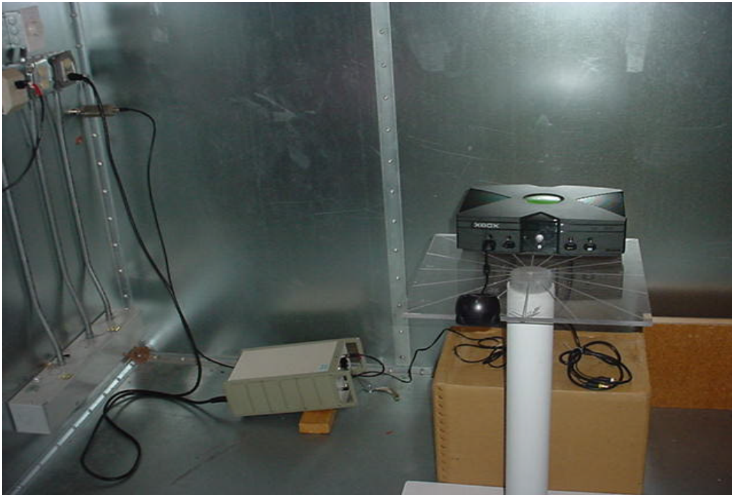
Conducted Emission Setup Overview
