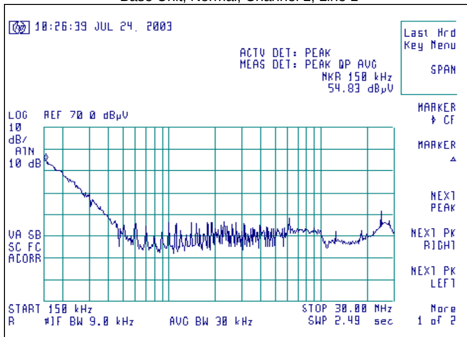
Signature Scan of Conducted Emissions Base Unit, Normal, Channel 1, Line 1
