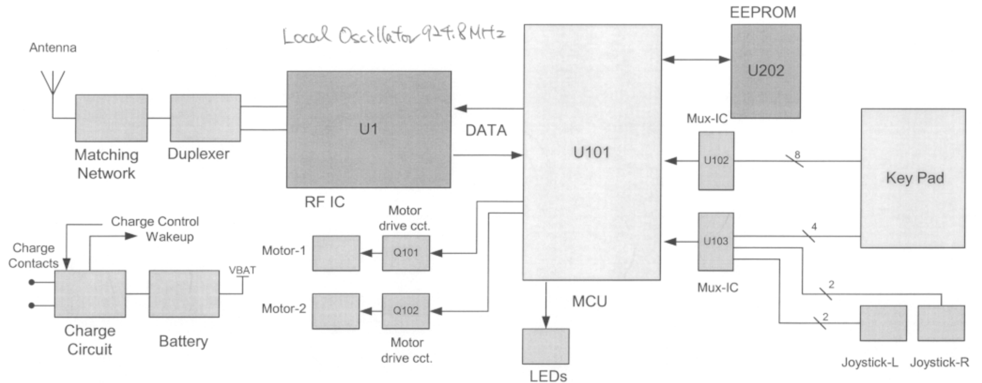
Sakura Controller Block Diagram
