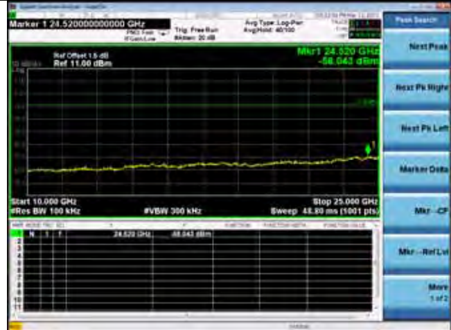
2441MHz(10GHz – 25GHz)
