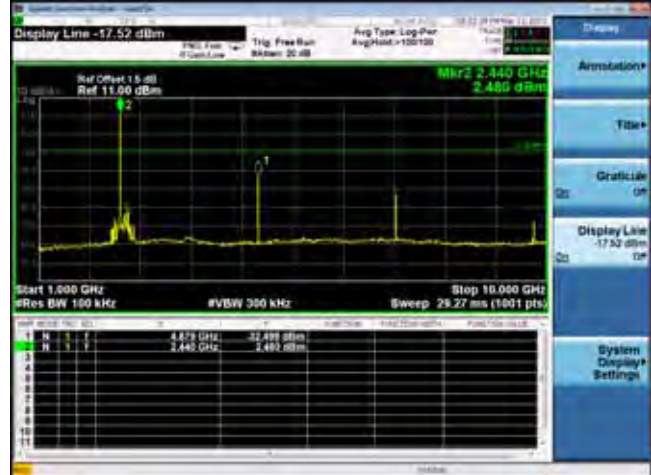
2441MHz(1GHz – 10GHz)
