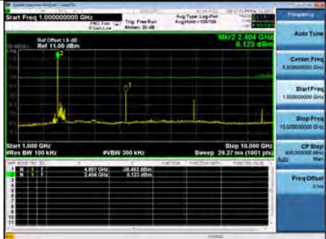
2402MHz(1GHz – 10GHz)
