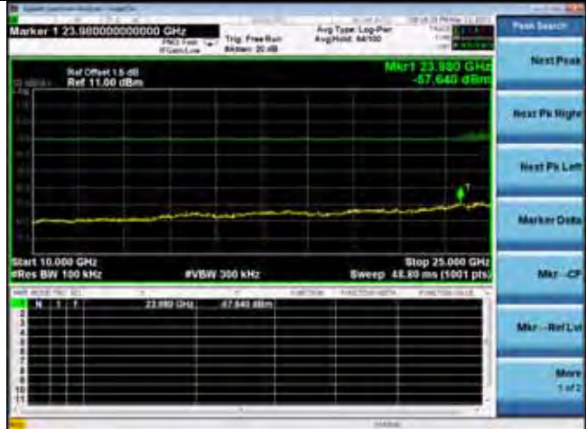
2402MHz(10GHz – 25GHz)
