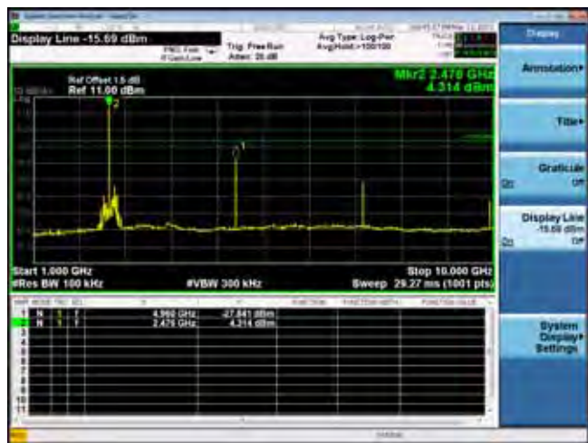
2480MHz(1GHz – 10GHz)
