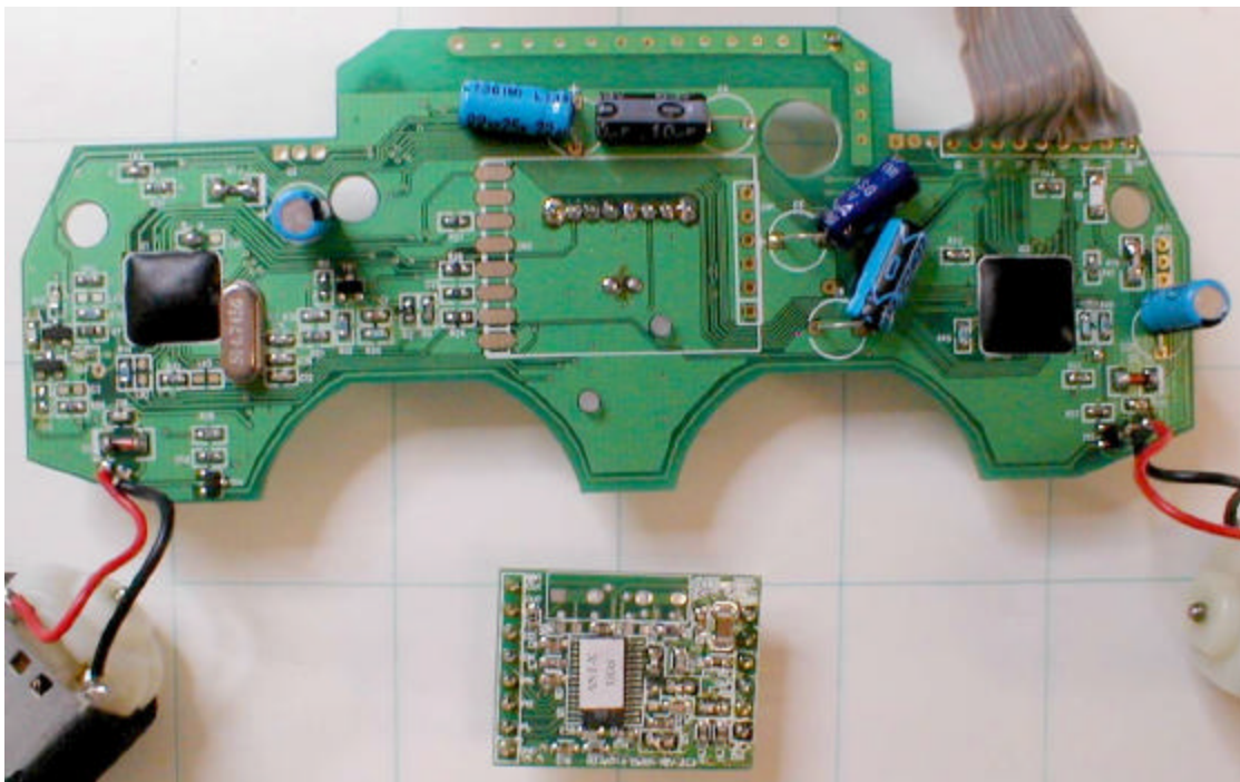
Main Board Top, ANT Module Removed
