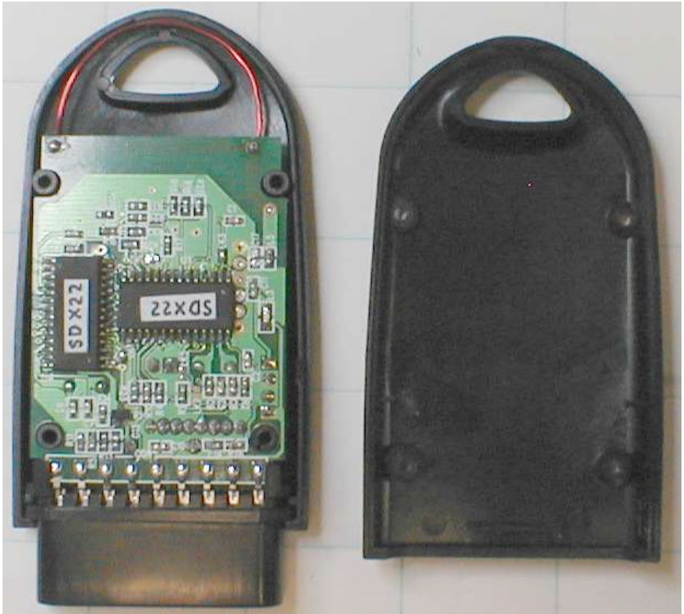
Cover Removed (Bottom View of Main PCB)
