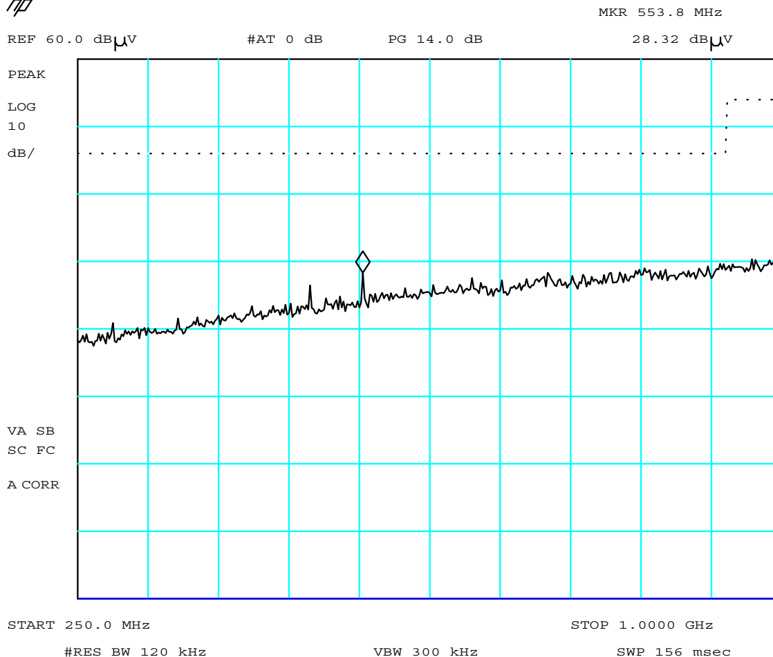
PLOT 7 Radiated Emissions - Peripherals Not Powered - 250MHz to 1GHz
