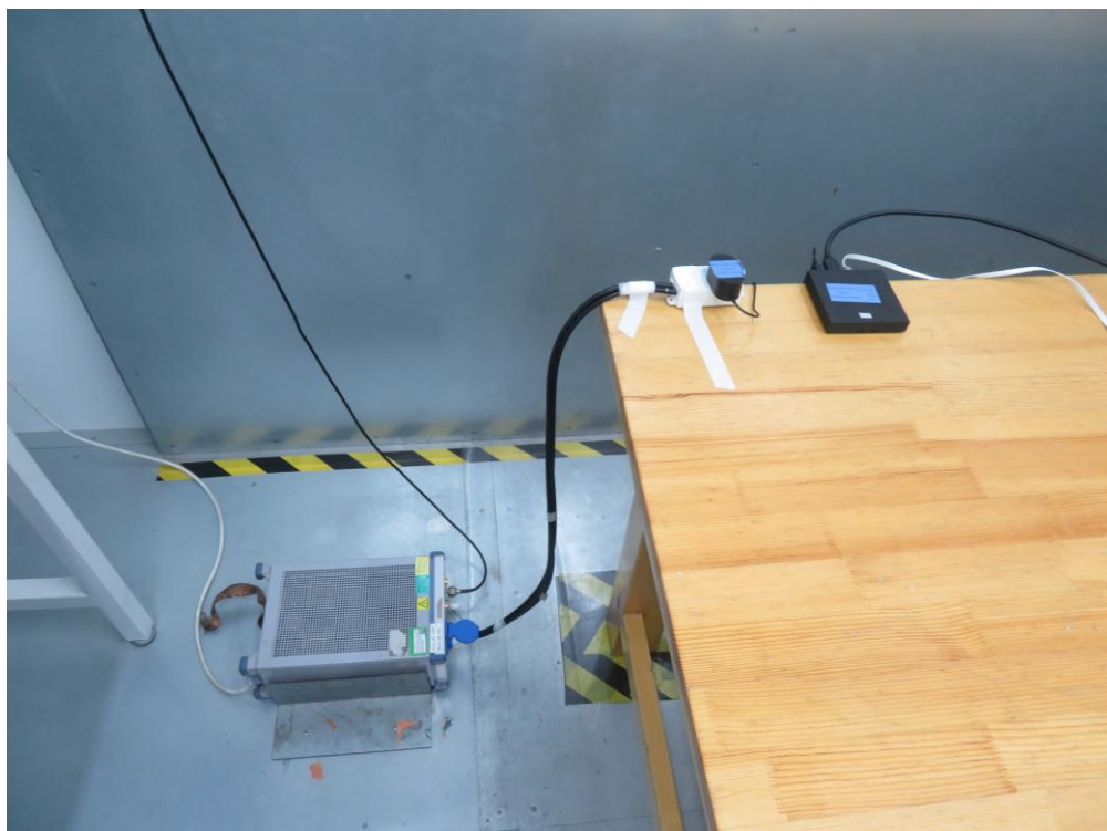
Description: Front View of AC Conducted Emission Test Setup
