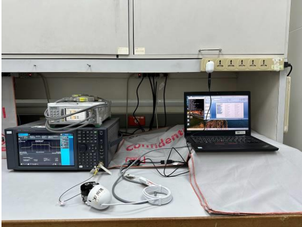
FCC_15_407_WLAN_Conducted_Setup
