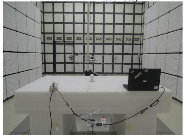
FCC_15_247_BLE_Radiated_Setup
