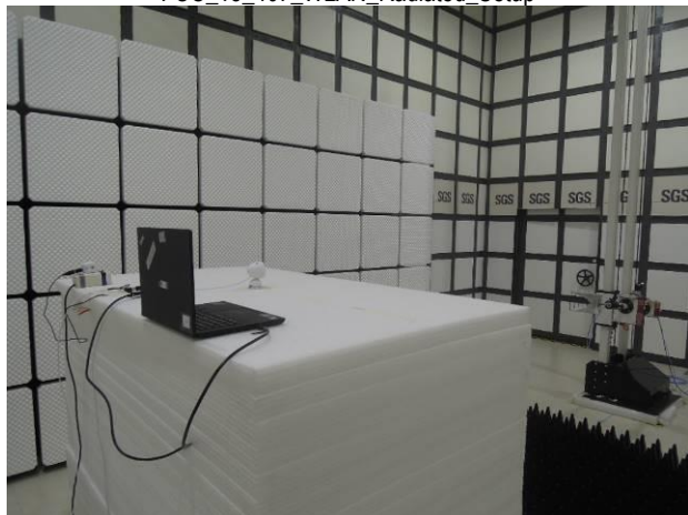
FCC_15_407_WLAN_Radiated_Setup
