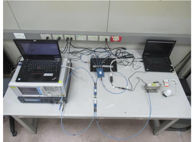
FCC_15_407_WLAN_Normal_DFS_Slave_Setup
