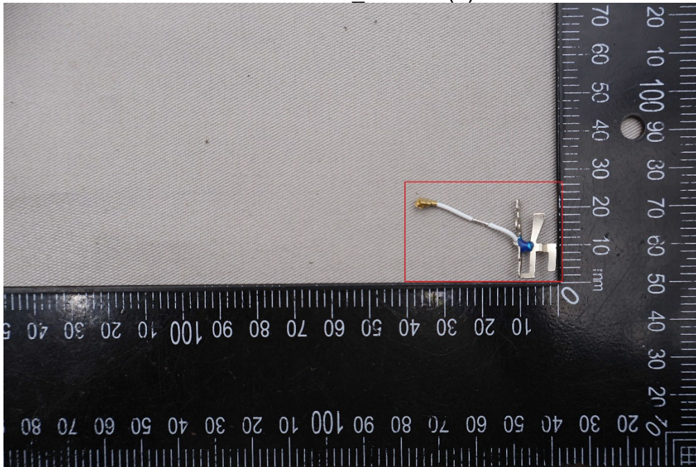
BLE&WLAN_Antenna(1)
