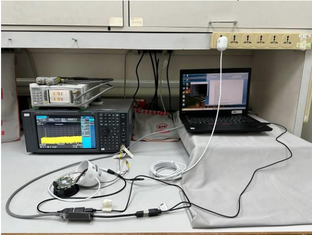
FCC_15_247_WLAN_Conducted_Setup
