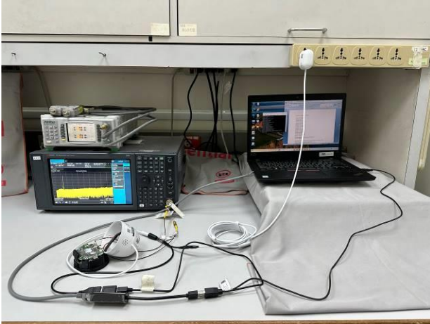
FCC_15_407_WLAN_Conducted_Setup
