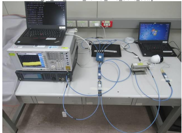
FCC_15_407_WLAN_Normal_DFS_Slave_Setup
