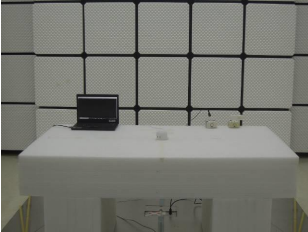
FCC 15 247 BLE Radiated Setup Spot Check
