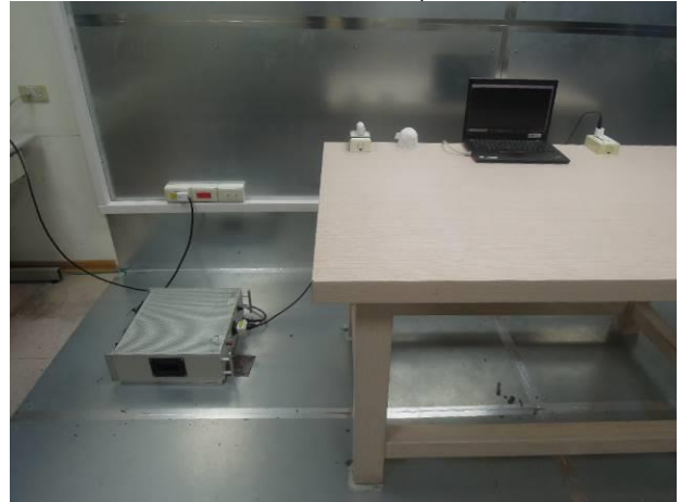
Conduction_Setup
