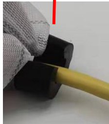
Assembly of waterproof circle (into the wateroppf connector)
