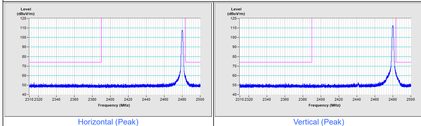
BT-LE 1M Channel 39
