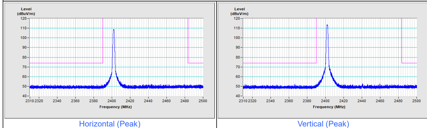
BT-LE 1M Channel 0
