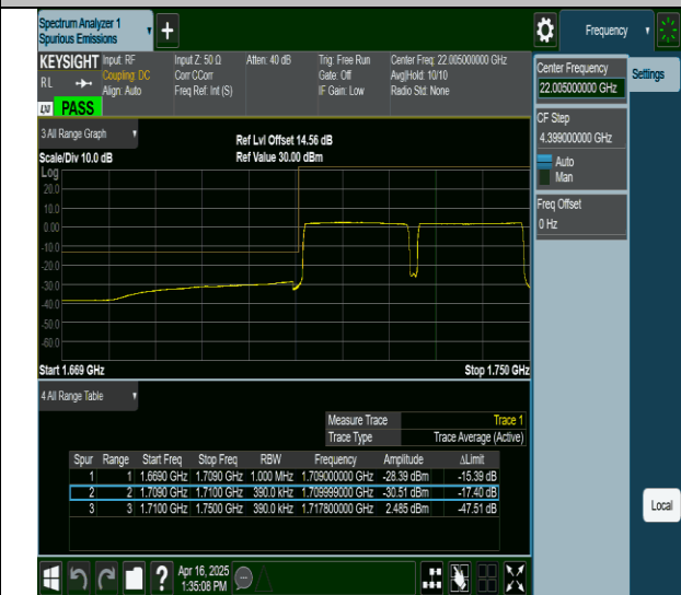
66-66-20MHz-20MHz-QPSK@QPSK-QPSK@QPSK-132072- 132270-100RB#0@0RB#0-100RB#0@0RB#0-PASS
