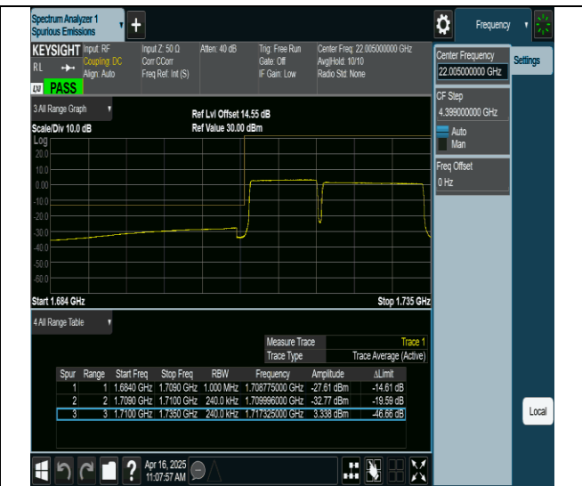
66-66-10MHz-15MHz-QPSK@QPSK-QPSK@QPSK-132025-132145-50RB#0@0RB#0-75RB#0@0RB#0-PASS
