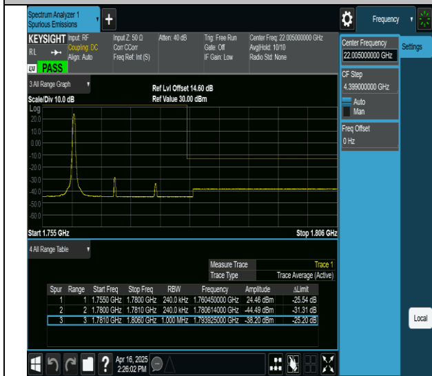
66-66-5MHz-20MHz-QPSK@QPSK-QPSK@QPSK-132455- 132572-1RB#24@0RB#0-0RB#0@0RB#0-PASS
