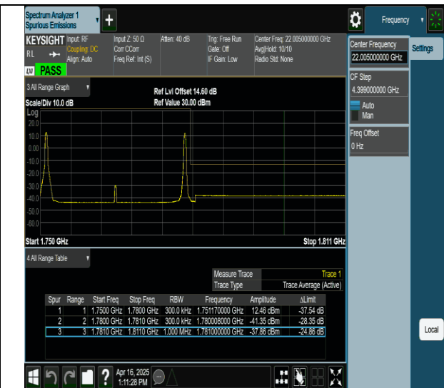
66-66-20MHz-10MHz-QPSK@QPSK-QPSK@QPSK-132473- 132617-1RB#0@0RB#0-1RB#49@0RB#0-PASS
