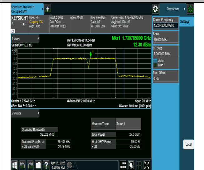
66-66-20MHz-15MHz-256QAM-256QAM-132072-132243-100RB#0-75RB#0-PASS
