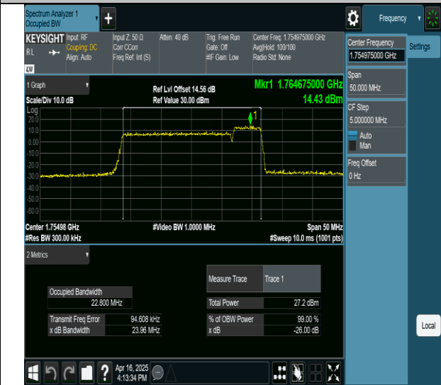
66-66-20MHz-5MHz-256QAM-256QAM-132397-132514-100RB#0-25RB#0-PASS
