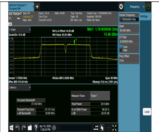
66-66-20MHz-20MHz-16QAM-16QAM-132323-132521-100RB#0-100RB#0-PASS
