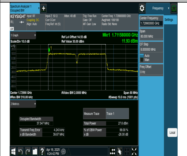
66-66-20MHz-20MHz-256QAM-256QAM-132072-132270-100RB#0-100RB#0-PASS
