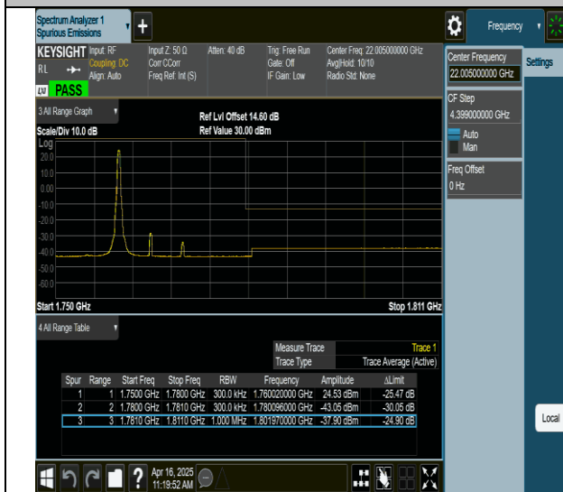
66-66-10MHz-20MHz-QPSK@QPSK-QPSK@QPSK-132428- 132572-1RB#49@0RB#0-0RB#0@0RB#0-PASS
