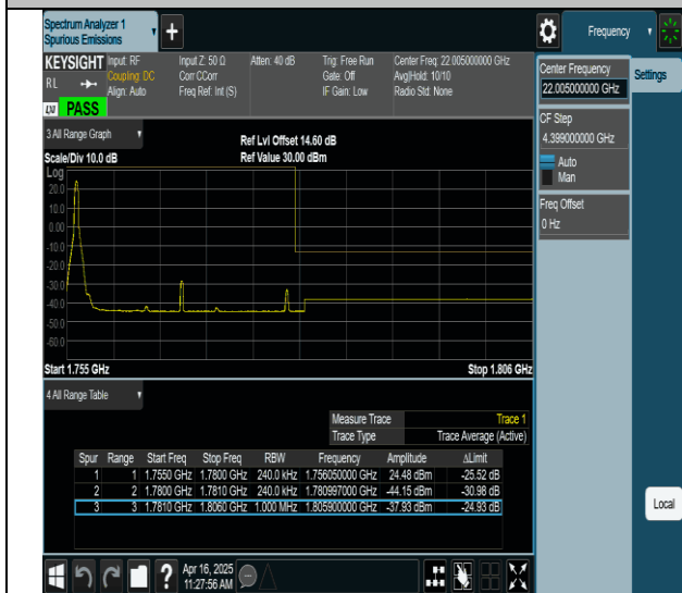
66-66-15MHz-10MHz-QPSK@QPSK-QPSK@QPSK-132499- 132619-1RB#0@0RB#0-0RB#0@0RB#0-PASS
