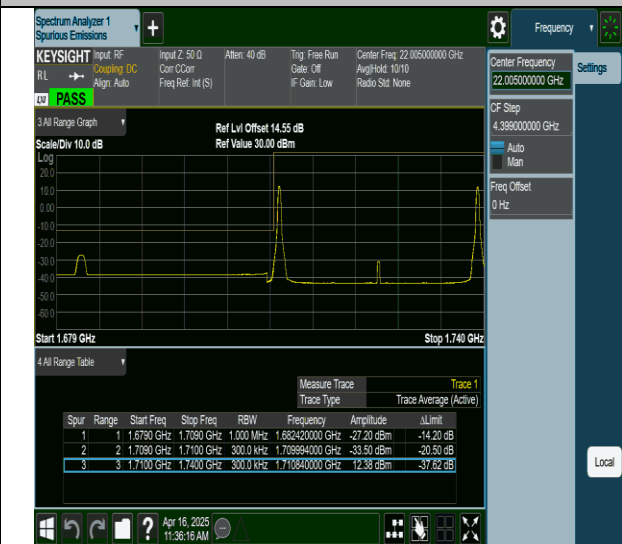
66-66-15MHz-15MHz-QPSK@QPSK-QPSK@QPSK-132047-132197-1RB#0@0RB#0-1RB#74@0RB#0-PASS
