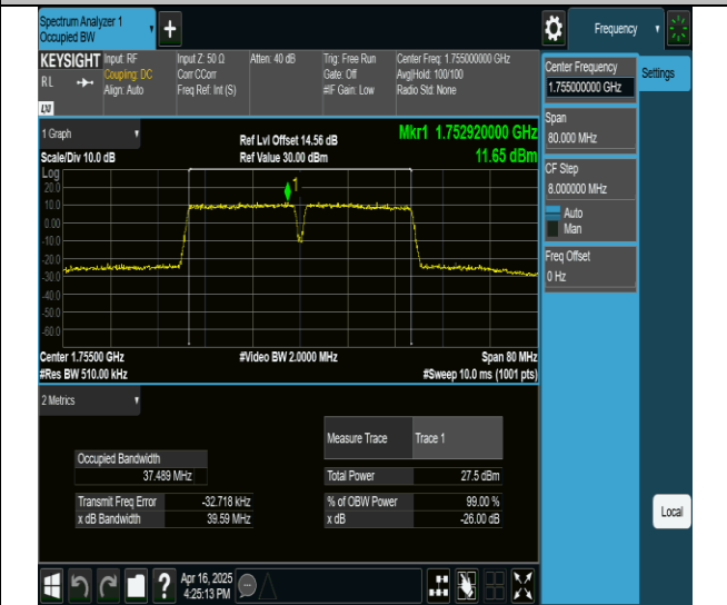
66-66-20MHz-20MHz-256QAM-256QAM-132323-132521-100RB#0-100RB#0-PASS
