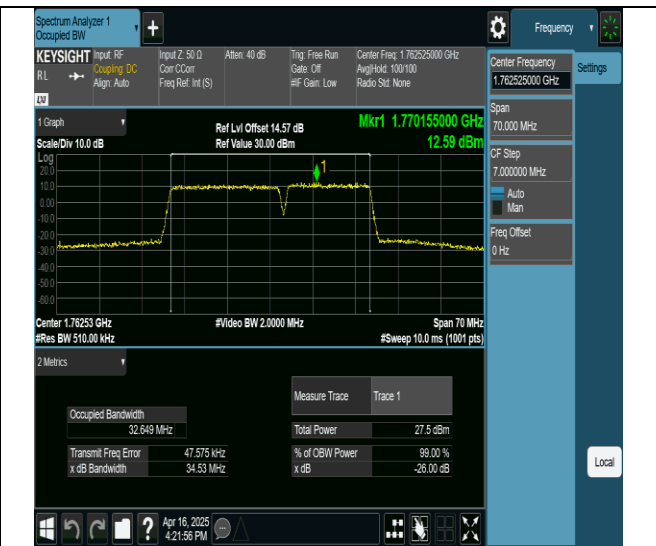
66-66-20MHz-15MHz-256QAM-256QAM-132423-132594-100RB#0-75RB#0-PASS
