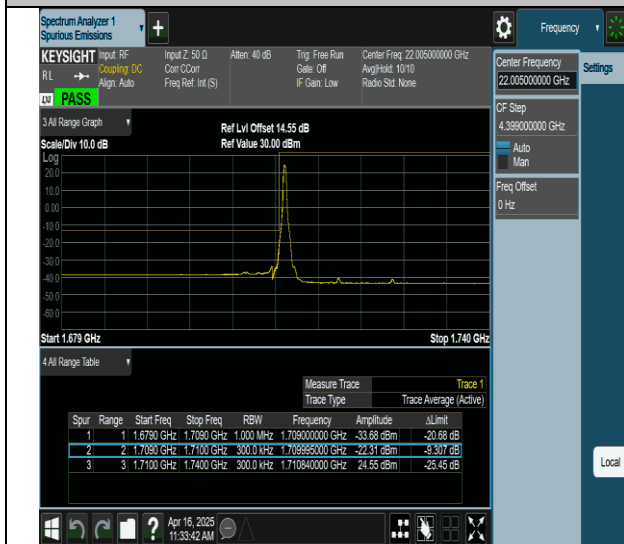
66-66-15MHz-15MHz-QPSK@QPSK-QPSK@QPSK-132047-132197-1RB#0@0RB#0-0RB#0@0RB#0-PASS
