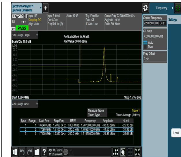
66-66-10MHz-15MHz-QPSK@QPSK-QPSK@QPSK-132025-132145-1RB#49@0RB#0-0RB#0@0RB#0-PASS
