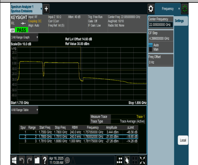
66-66-10MHz-15MHz-QPSK@QPSK-QPSK@QPSK-132477-132597-50RB#0@0RB#0-75RB#0@0RB#0-PASS
