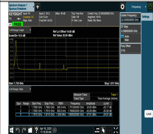
66-66-10MHz-20MHz-QPSK@QPSK-QPSK@QPSK-132428- 132572-1RB#0@0RB#0-0RB#0@0RB#0-PASS
