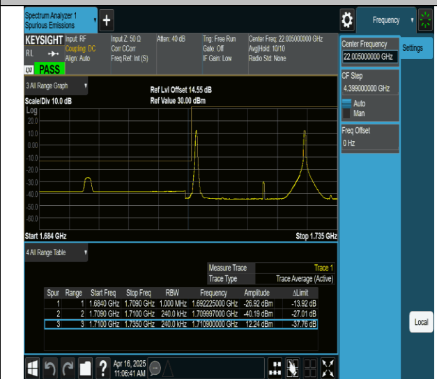
66-66-10MHz-15MHz-QPSK@QPSK-QPSK@QPSK-132025- 132145-1RB#0@0RB#0-1RB#49@0RB#0-PASS
