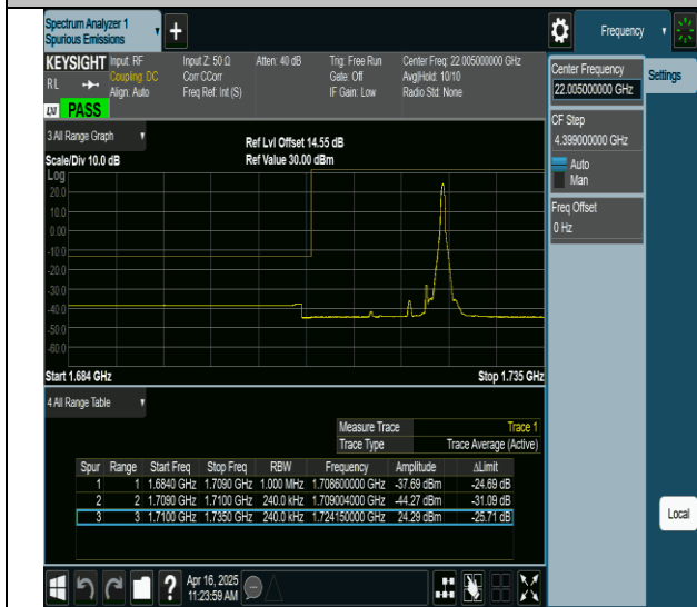
66-66-15MHz-10MHz-QPSK@QPSK-QPSK@QPSK-132047- 132167-1RB#74@0RB#0-0RB#0@0RB#0-PASS
