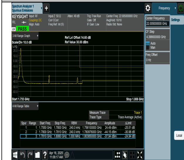
66-66-10MHz-15MHz-QPSK@QPSK-QPSK@QPSK-132477-132597-1RB#0@0RB#0-0RB#0@0RB#0-PASS
