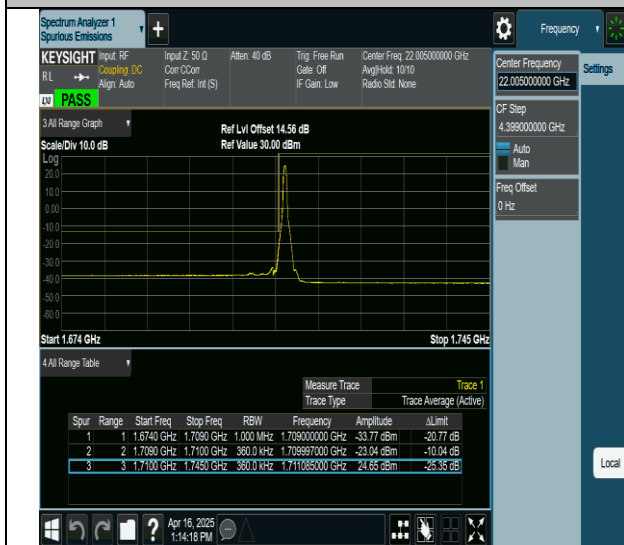
66-66-20MHz-15MHz-QPSK@QPSK-QPSK@QPSK-132072- 132243-1RB#0@0RB#0-0RB#0@0RB#0-PASS
