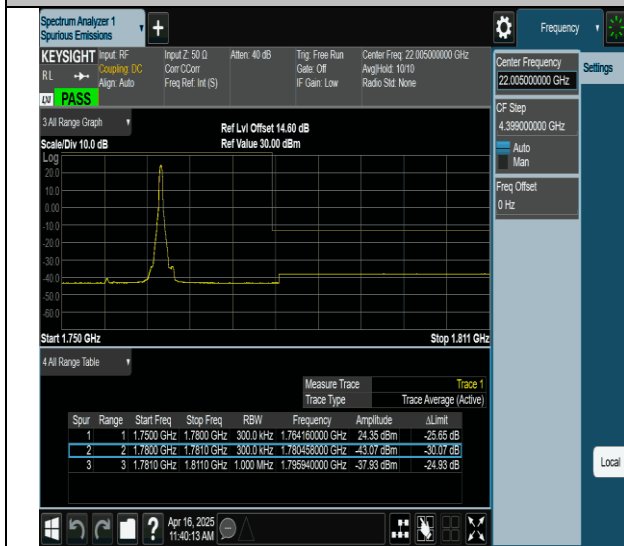
66-66-15MHz-15MHz-QPSK@QPSK-QPSK@QPSK-132447- 132597-1RB#74@0RB#0-0RB#0@0RB#0-PASS
