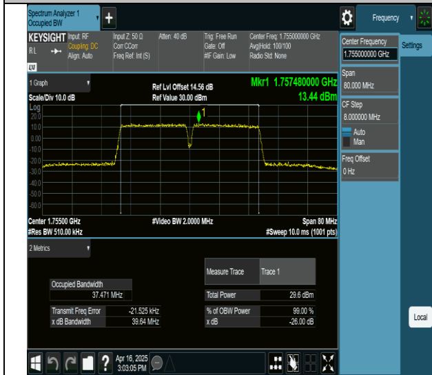
66-66-20MHz-20MHz-64QAM-64QAM-132323-132521-100RB#0-100RB#0-PASS
