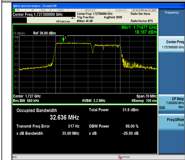
66-66-20MHz-15MHz-QPSK-QPSK-132072-132243-100RB#0-75RB#0-PASS
