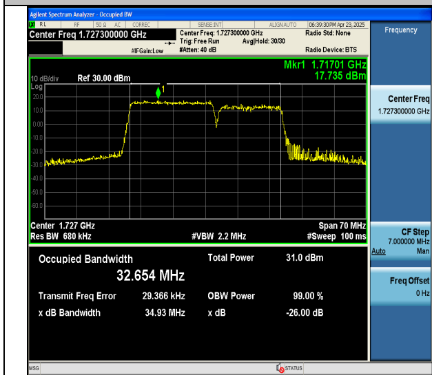
66-66-20MHz-15MHz-64QAM-64QAM-132072-132243-100RB#0-75RB#0-PASS
