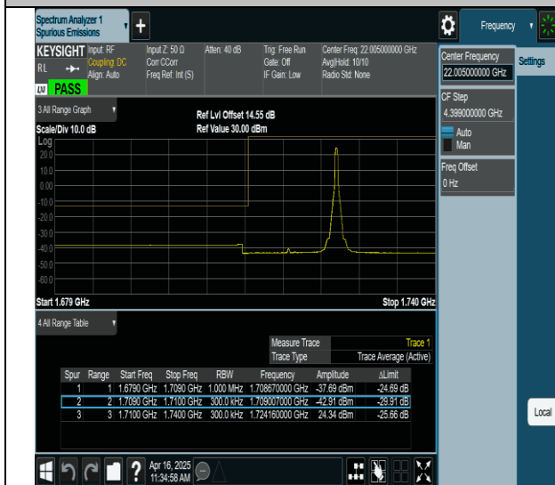
66-66-15MHz-15MHz-QPSK@QPSK-QPSK@QPSK-132047-132197-1RB#74@0RB#0-0RB#0@0RB#0-PASS
