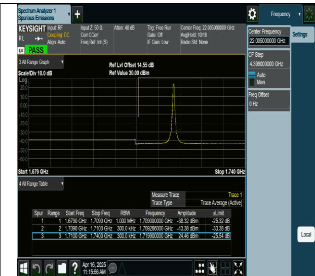
66-66-10MHz-20MHz-QPSK@QPSK-QPSK@QPSK-132027- 132171-1RB#49@0RB#0-0RB#0@0RB#0-PASS
