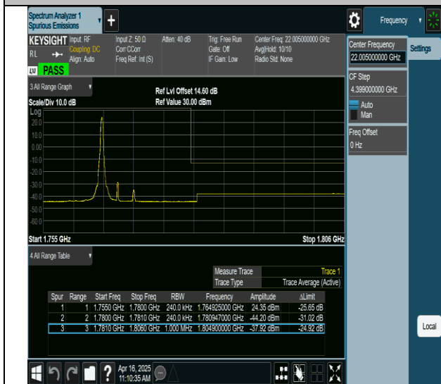
66-66-10MHz-15MHz-QPSK@QPSK-QPSK@QPSK-132477-132597-1RB#49@0RB#0-0RB#0@0RB#0-PASS
