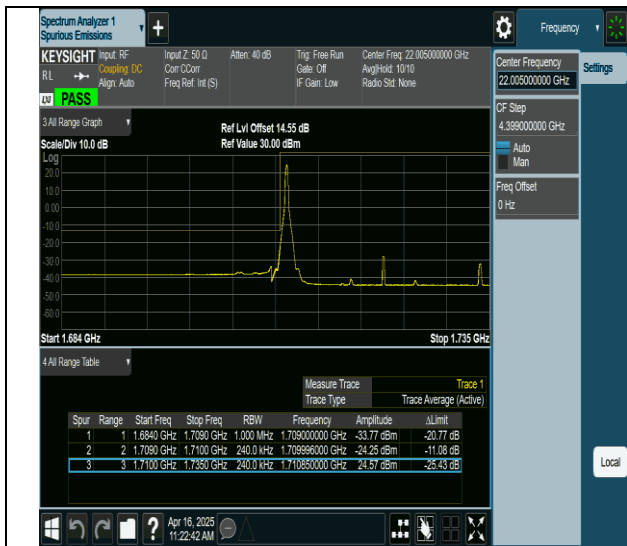
66-66-15MHz-10MHz-QPSK@QPSK-QPSK@QPSK-132047- 132167-1RB#0@0RB#0-0RB#0@0RB#0-PASS
