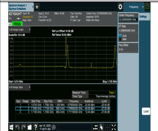
66-66-15MHz-20MHz-QPSK@QPSK-QPSK@QPSK-132050- 132221-1RB#0@0RB#0-1RB#99@0RB#0-PASS
