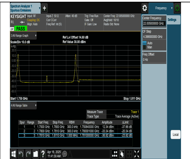
66-66-15MHz-15MHz-QPSK@QPSK-QPSK@QPSK-132447- 132597-1RB#0@0RB#0-1RB#74@0RB#0-PASS
