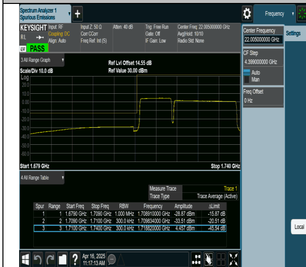
66-66-10MHz-20MHz-QPSK@QPSK-QPSK@QPSK-132027- 132171-50RB#0@0RB#0-100RB#0@0RB#0-PASS
