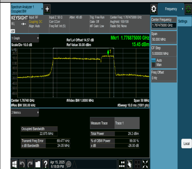
66-66-20MHz-5MHz-16QAM-16QAM-132522-132639-100RB#0-25RB#0-PASS
