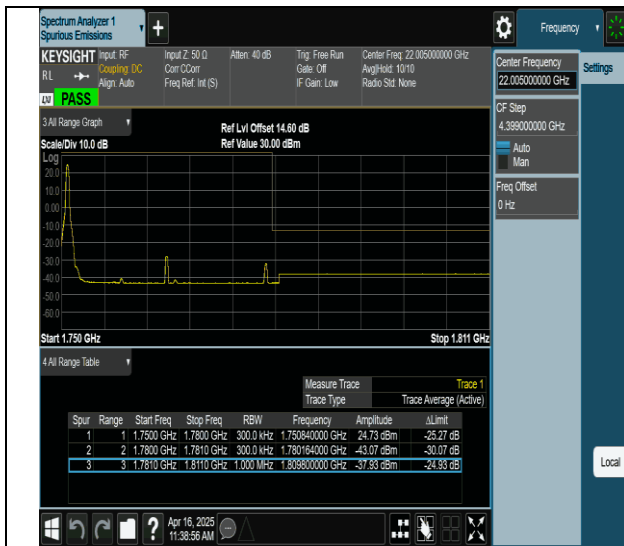
66-66-15MHz-15MHz-QPSK@QPSK-QPSK@QPSK-132447- 132597-1RB#0@0RB#0-0RB#0@0RB#0-PASS
