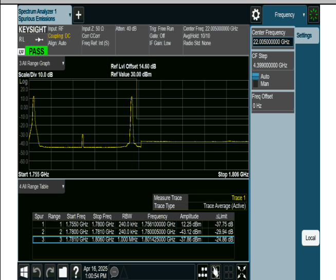
66-66-20MHz-5MHz-QPSK@QPSK-QPSK@QPSK-132522-132639-1RB#0@0RB#0-1RB#24@0RB#0-PASS
