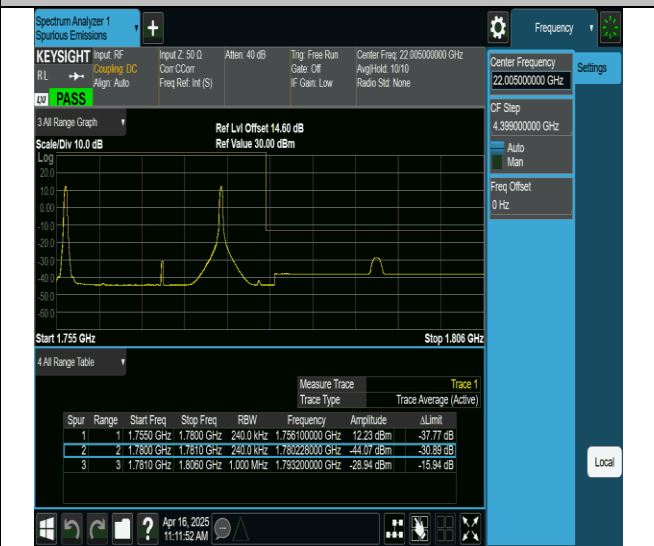
66-66-10MHz-15MHz-QPSK@QPSK-QPSK@QPSK-132477-132597-1RB#0@0RB#0-1RB#49@0RB#0-PASS
