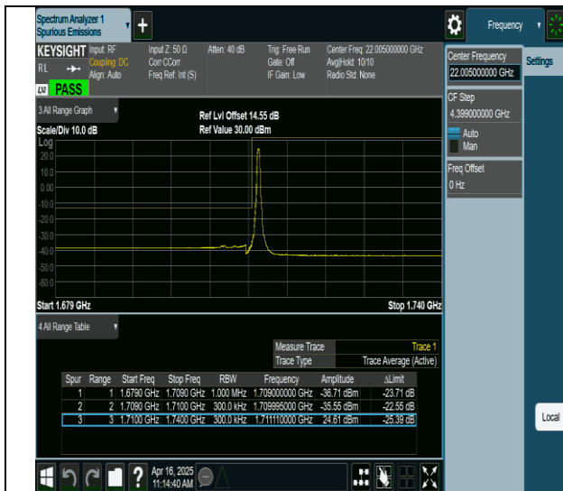
66-66-10MHz-20MHz-QPSK@QPSK-QPSK@QPSK-132027- 132171-1RB#0@0RB#0-0RB#0@0RB#0-PASS
