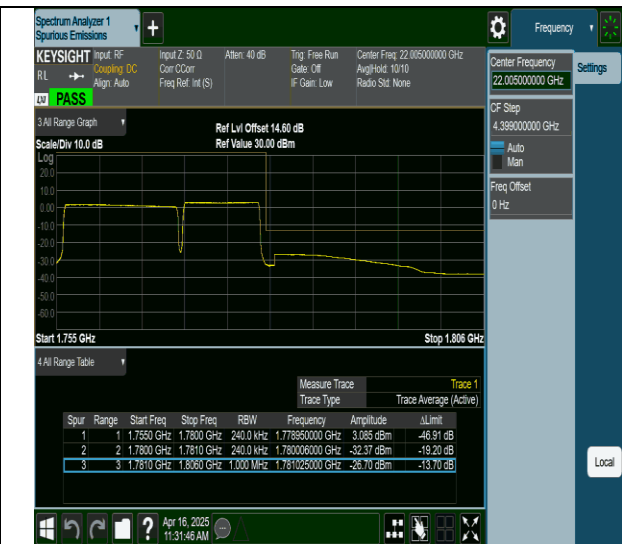
66-66-15MHz-10MHz-QPSK@QPSK-QPSK@QPSK-132499-132619-75RB#0@0RB#0-50RB#0@0RB#0-PASS
