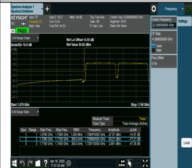
66-66-15MHz-15MHz-QPSK@QPSK-QPSK@QPSK-132047-132197-75RB#0@0RB#0-75RB#0@0RB#0-PASS
