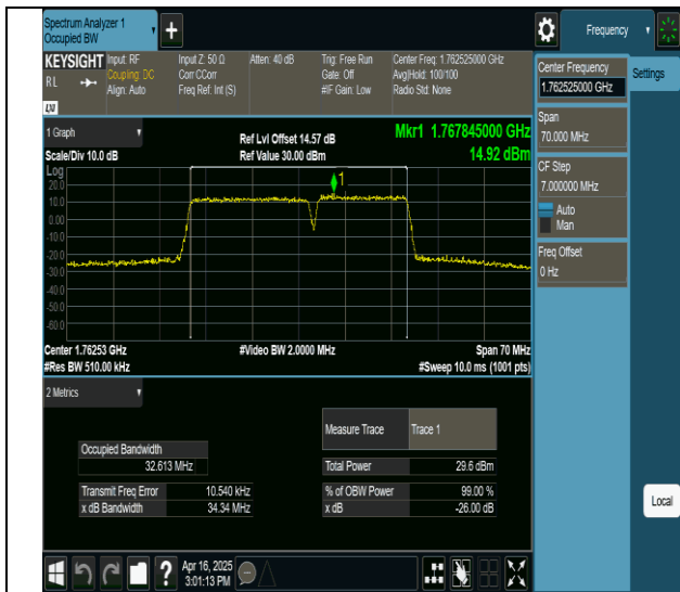
66-66-20MHz-15MHz-64QAM-64QAM-132423-132594-100RB#0-75RB#0-PASS
