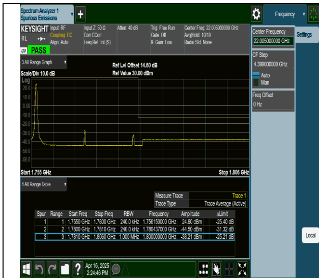
66-66-5MHz-20MHz-QPSK@QPSK-QPSK@QPSK-132455- 132572-1RB#0@0RB#0-0RB#0@0RB#0-PASS
