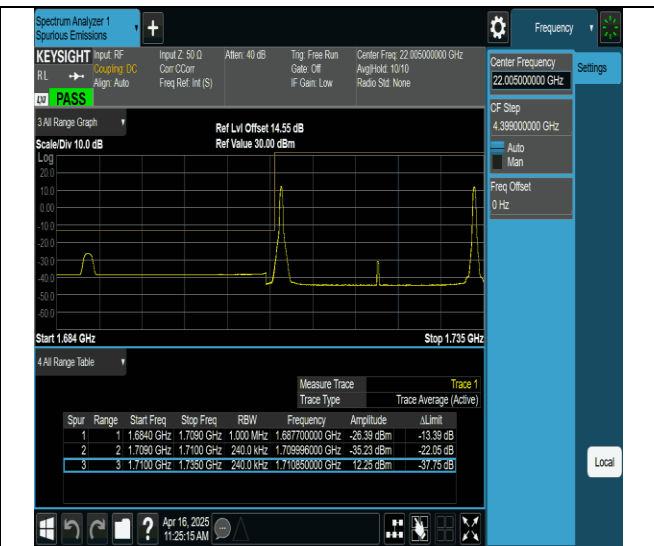
66-66-15MHz-10MHz-QPSK@QPSK-QPSK@QPSK-132047- 132167-1RB#0@0RB#0-1RB#49@0RB#0-PASS
