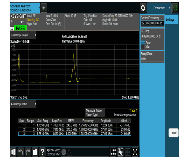
66-66-5MHz-20MHz-QPSK@QPSK-QPSK@QPSK-132455- 132572-1RB#0@0RB#0-1RB#99@0RB#0-PASS
