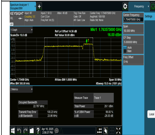
66-66-20MHz-5MHz-64QAM-64QAM-132397-132514-100RB#0-25RB#0-PASS
