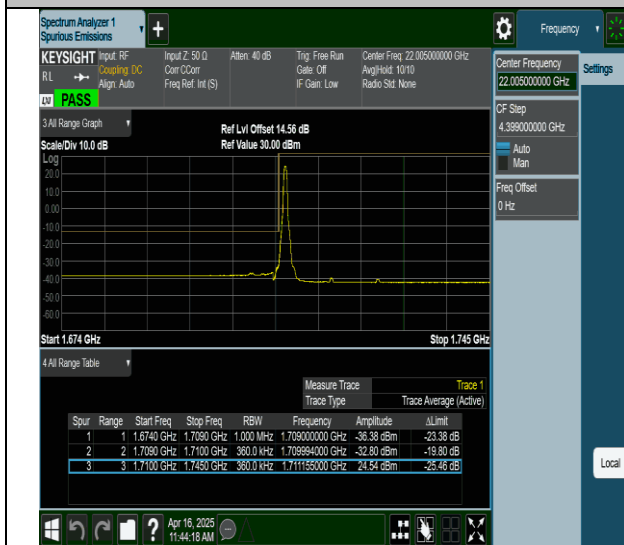
66-66-15MHz-20MHz-QPSK@QPSK-QPSK@QPSK-132050- 132221-1RB#0@0RB#0-0RB#0@0RB#0-PASS
