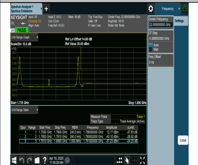
66-66-15MHz-10MHz-QPSK@QPSK-QPSK@QPSK-132499- 132619-1RB#0@0RB#0-1RB#49@0RB#0-PASS
