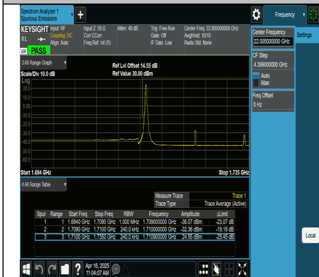
66-66-10MHz-15MHz-QPSK@QPSK-QPSK@QPSK-132025- 132145-1RB#0@0RB#0-0RB#0@0RB#0-PASS
