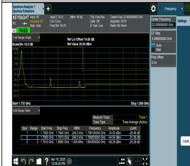
66-66-20MHz-5MHz-QPSK@QPSK-QPSK@QPSK-132522-132639-1RB#0@0RB#0-0RB#0@0RB#0-PASS
