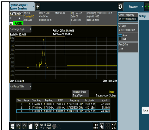
66-66-15MHz-10MHz-QPSK@QPSK-QPSK@QPSK-132499-132619-1RB#74@0RB#0-0RB#0-PASS
