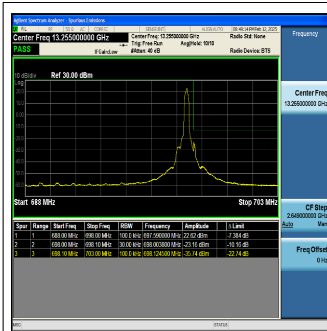
NTNV-n71-PC3-15-10-H-DFT-BPSK-Edge_1RB_Right-PASS
