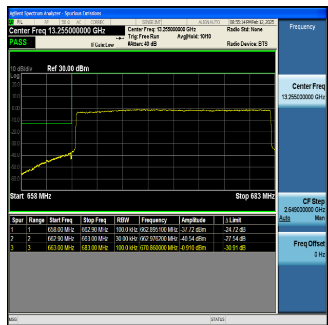
NTNV-n71-PC3-15-20-L-CP-QPSK-Outer_Full-PASS
