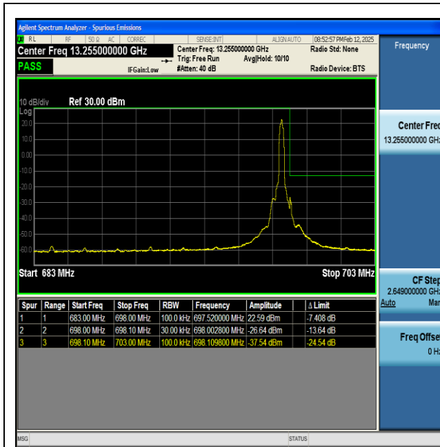
NTNV-n71-PC3-15-15-H-DFT-BPSK-Edge_1RB_Right-PASS
