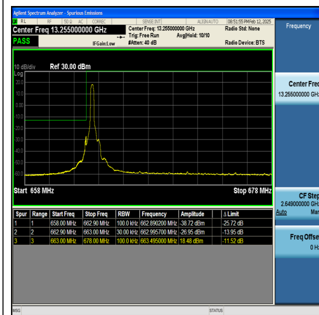
NTNV-n71-PC3-15-15-L-CP-QPSK-Edge_1RB_Left-PASS
