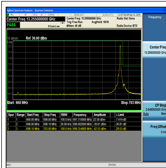
NTNV-n71-PC3-15-30-H-DFT-BPSK-Edge_1RB_Right-PASS
