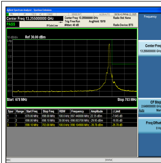
NTNV-n71-PC3-15-20-H-DFT-BPSK-Edge_1RB_Right-PASS
