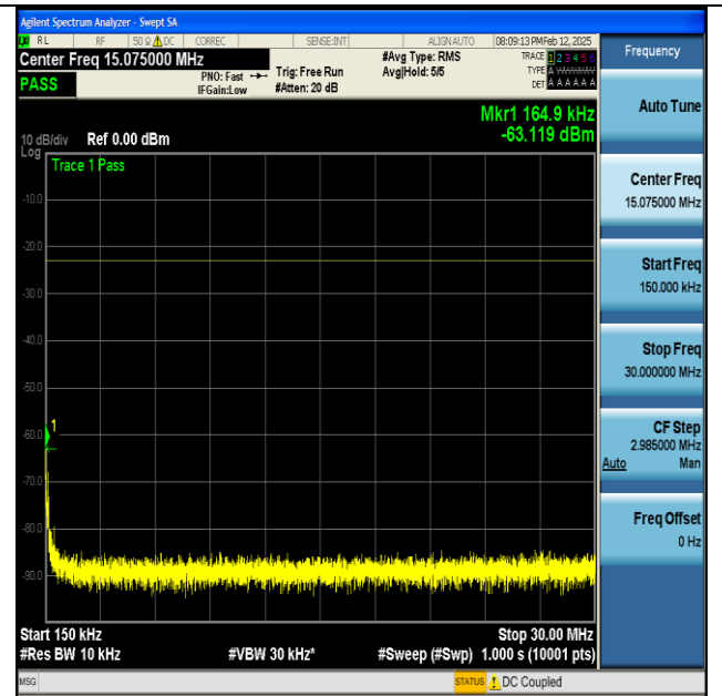
NTNV-n71-PC3-15-20-M-DFT-BPSK-Edge_1RB_Left- 0.15-30-PASS
