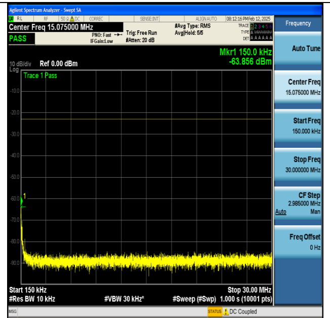
NTNV-n71-PC3-15-20-H-DFT-BPSK-Edge_1RB_Left-0.15- 30-PASS
