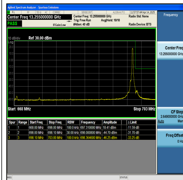
NTNV-n71-PC3-15-30-H-CP-QPSK-Edge_1RB_Right-PASS
