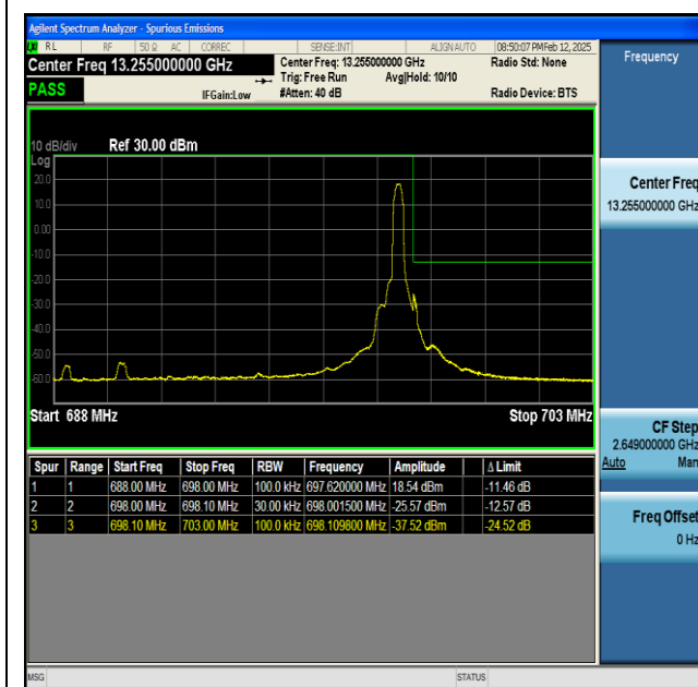
NTNV-n71-PC3-15-10-H-CP-QPSK-Edge_1RB_Right-PASS
