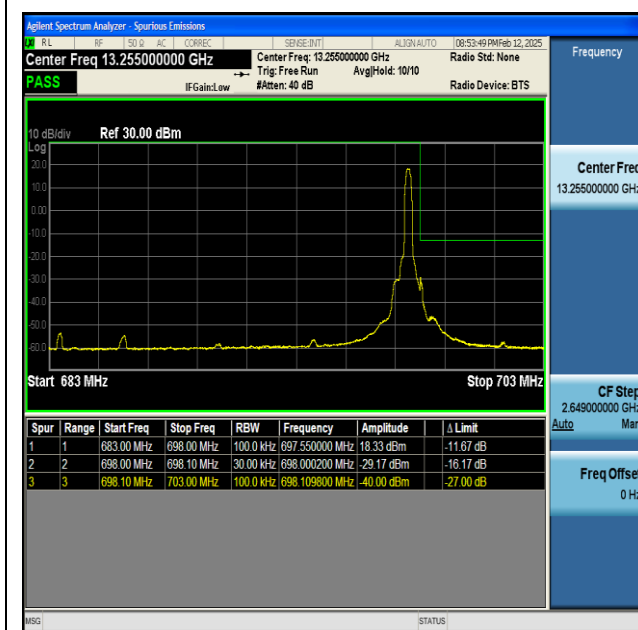
NTNV-n71-PC3-15-15-H-CP-QPSK-Edge_1RB_Right-PASS
