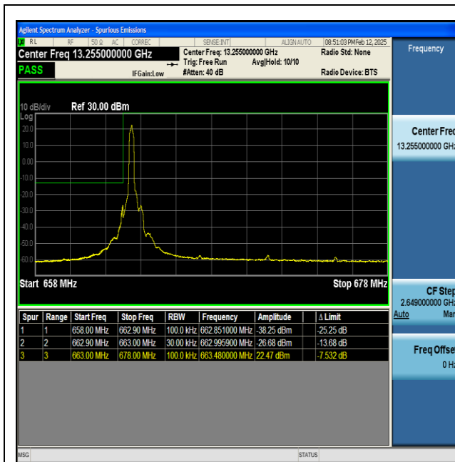
NTNV-n71-PC3-15-15-L-DFT-BPSK-Edge_1RB_Left-PASS
