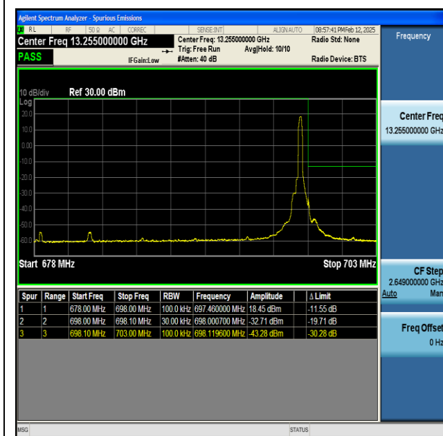
NTNV-n71-PC3-15-20-H-CP-QPSK-Edge_1RB_Right-PASS
