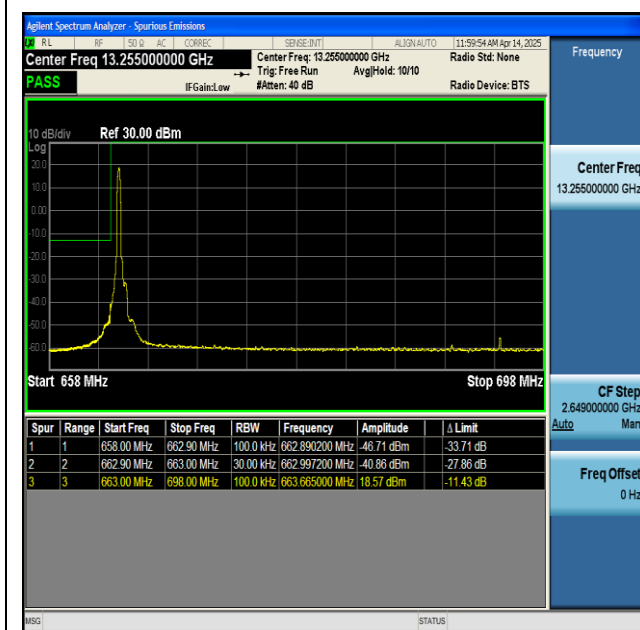
NTNV-n71-PC3-15-35-L-CP-QPSK-Edge_1RB_Left-PASS
