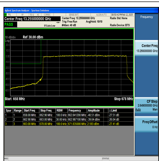
NTNV-n71-PC3-15-15-L-DFT-BPSK-Outer_Full-PASS
