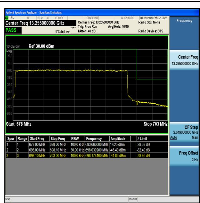
NTNV-n71-PC3-15-20-H-DFT-BPSK-Outer_Full-PASS
