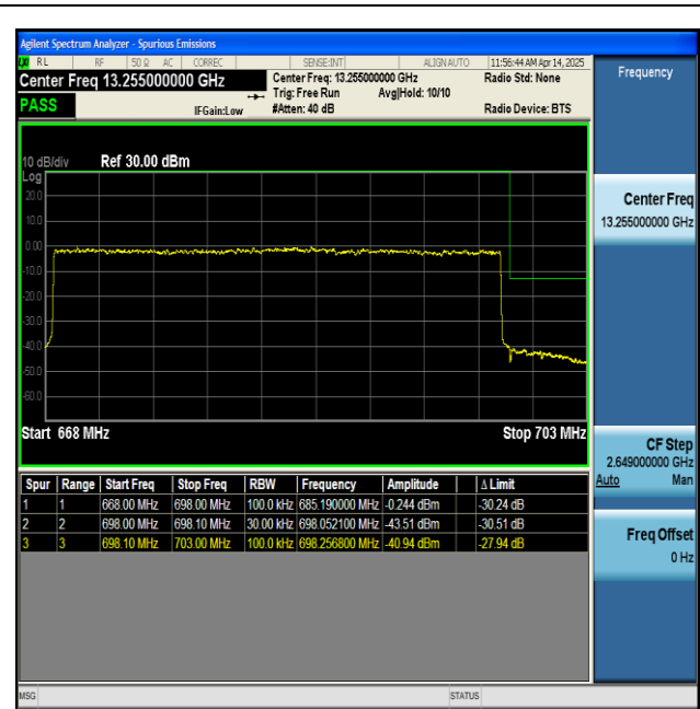
NTNV-n71-PC3-15-30-H-DFT-BPSK-Outer_Full-PASS
