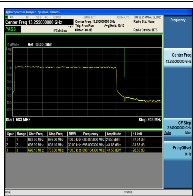
NTNV-n71-PC3-15-15-H-DFT-BPSK-Outer_Full-PASS
