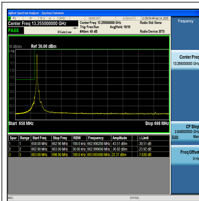
NTNV-n71-PC3-15-35-L-DFT-BPSK-Edge_1RB_Left-PASS
