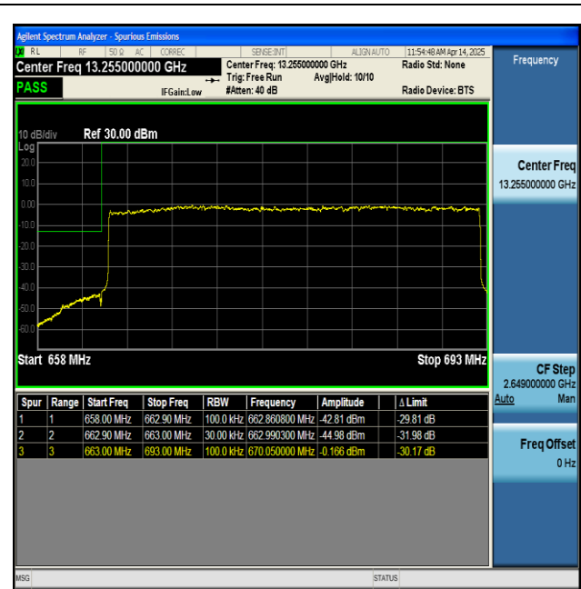
NTNV-n71-PC3-15-30-L-DFT-BPSK-Outer_Full-PASS
