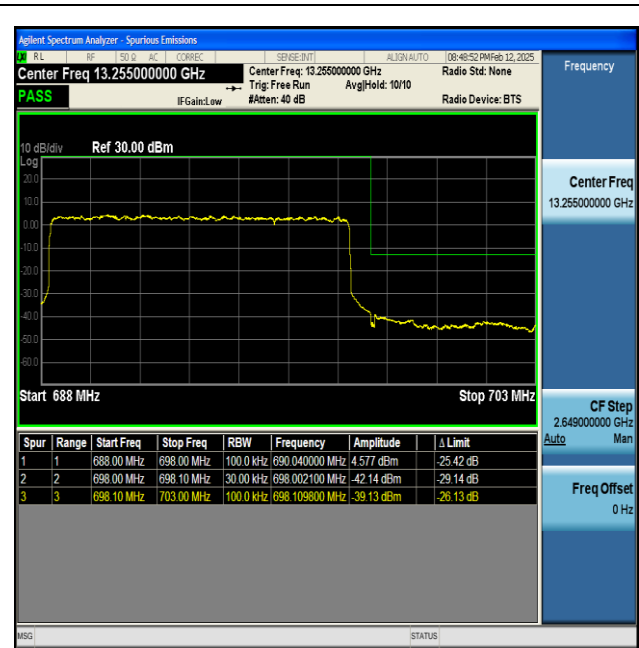
NTNV-n71-PC3-15-10-H-DFT-BPSK-Outer_Full-PASS
