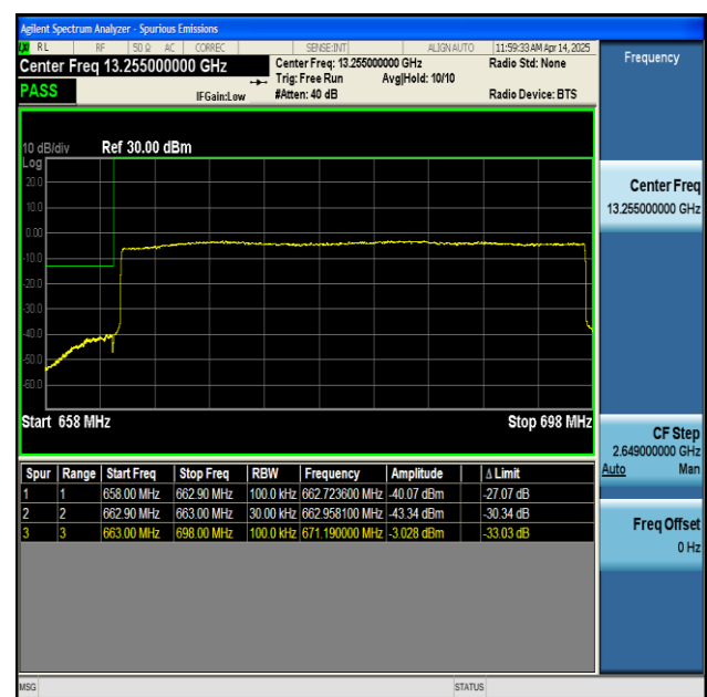
NTNV-n71-PC3-15-35-L-CP-QPSK-Outer_Full-PASS
