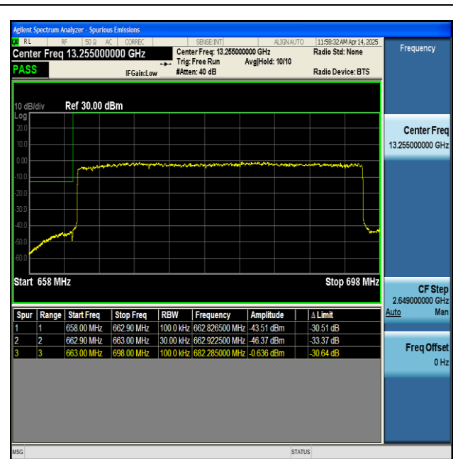
NTNV-n71-PC3-15-35-L-DFT-BPSK-Outer_Full-PASS
