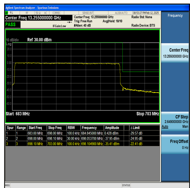
NTNV-n71-PC3-15-15-H-CP-QPSK-Outer_Full-PASS
