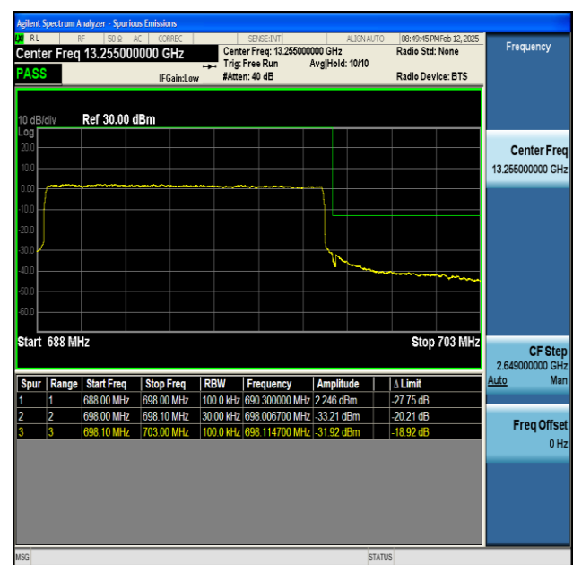
NTNV-n71-PC3-15-10-H-CP-QPSK-Outer_Full-PASS
