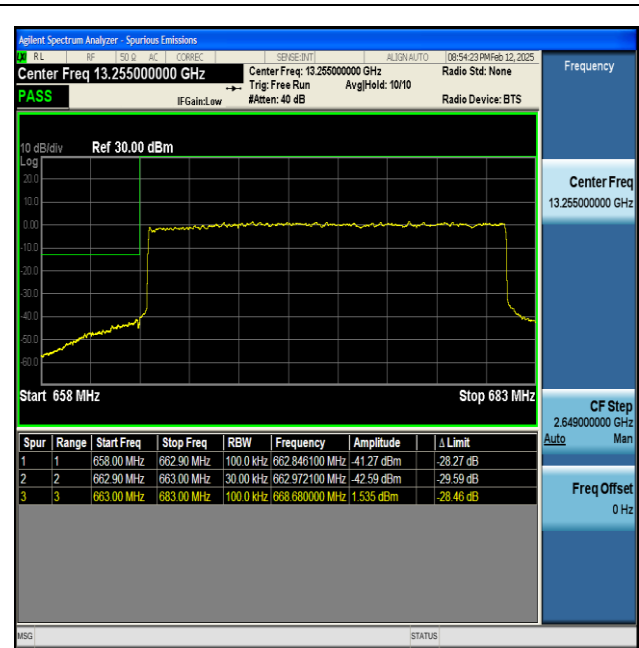
NTNV-n71-PC3-15-20-L-DFT-BPSK-Outer_Full-PASS
