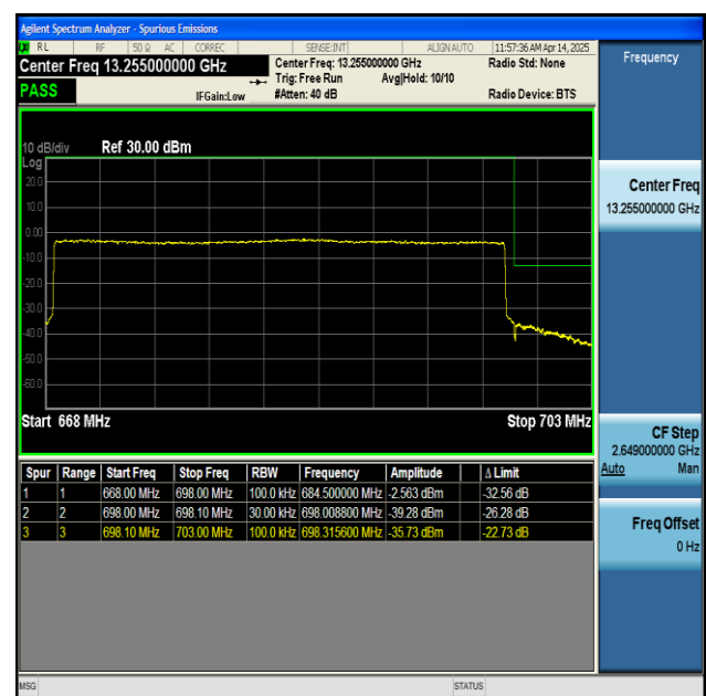
NTNV-n71-PC3-15-30-H-CP-QPSK-Outer_Full-PASS
