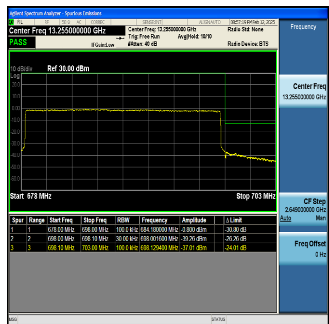
NTNV-n71-PC3-15-20-H-CP-QPSK-Outer_Full-PASS
