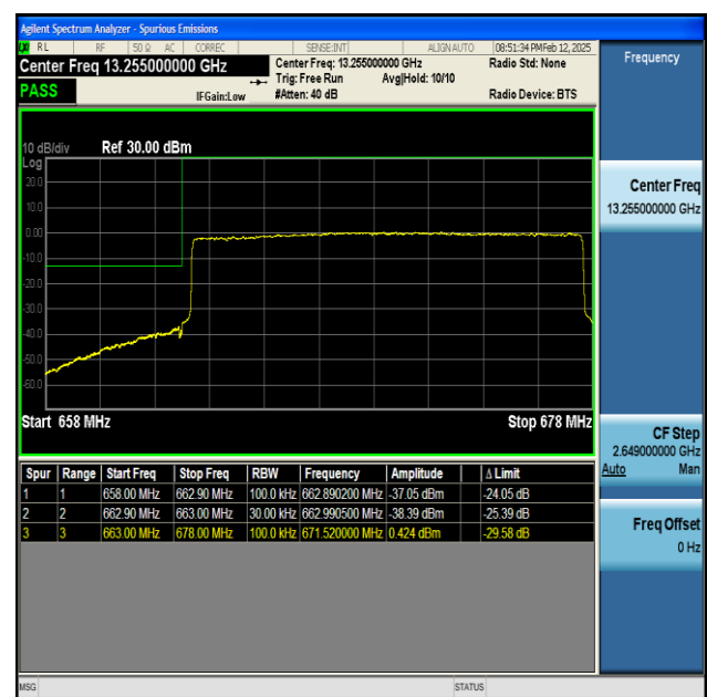
NTNV-n71-PC3-15-15-L-CP-QPSK-Outer_Full-PASS
