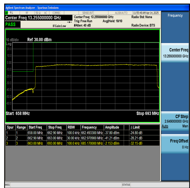
NTNV-n71-PC3-15-30-L-CP-QPSK-Outer_Full-PASS
