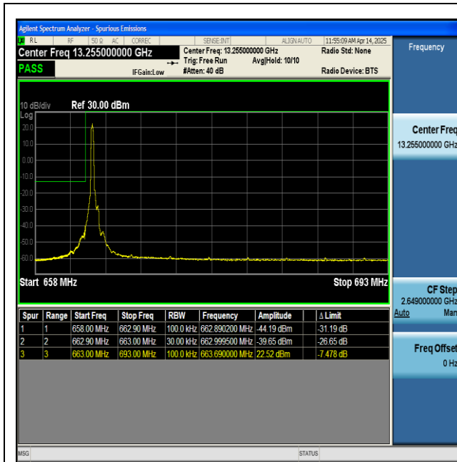
NTNV-n71-PC3-15-30-L-DFT-BPSK-Edge_1RB_Left-PASS
