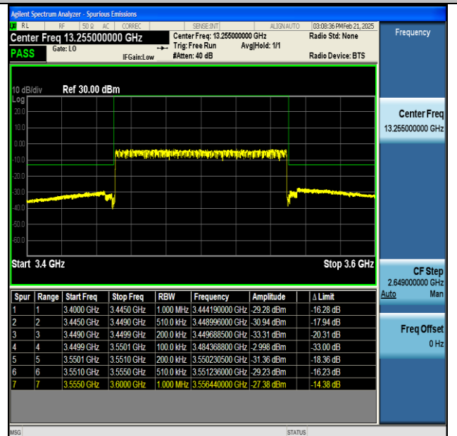
NTNV-n77(3450-3550)-PC2-30-100-L-CP-QPSK- Outer_Full-PASS
