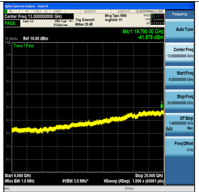
NTNV-n77(3450-3550)-PC2-30-100-M-DFT-BPSK- Edge_1RB_Left-6000-20000-PASS
