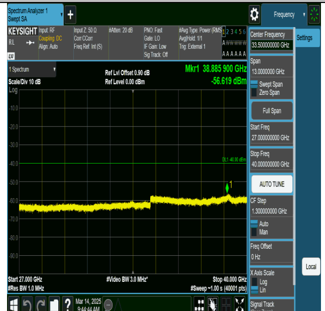
NTNV-n77(3450-3550)-PC2-30-100-L-CP-QPSK- Edge_1RB_Left-27000-40000-PASS
