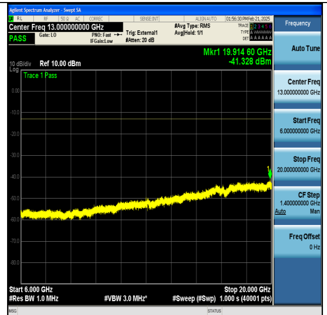
NTNV-n77(3450-3550)-PC2-30-100-L-CP-QPSK- Edge_1RB_Left-6000-20000-PASS
