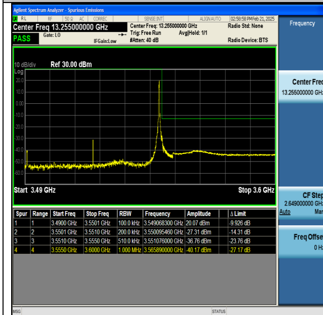
NTNV-n77(3450-3550)-PC2-30-60-H-CP-QPSK- Edge_1RB_Right-PASS
