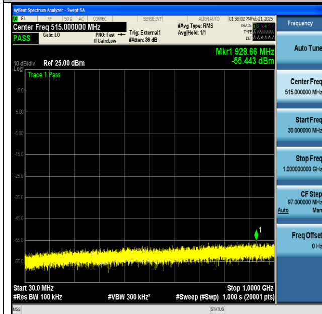
NTNV-n77(3450-3550)-PC2-30-100-M-DFT-BPSK- Edge_1RB_Left-30-1000-PASS
