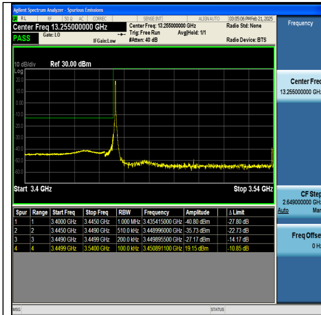
NTNV-n77(3450-3550)-PC2-30-90-L-DFT-BPSK- Edge_1RB_Left-PASS
