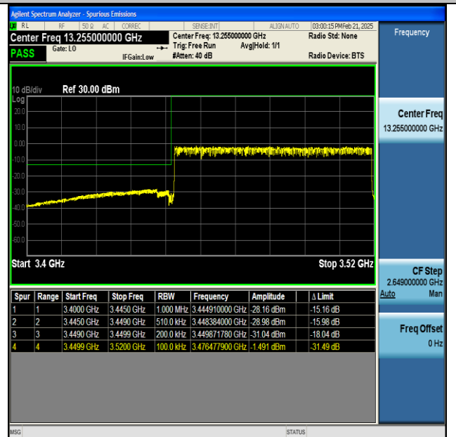
NTNV-n77(3450-3550)-PC2-30-70-L-CP-QPSK- Outer_Full-PASS
