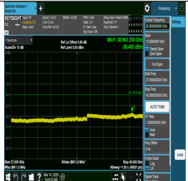
NTNV-n77(3450-3550)-PC2-30-100-L-DFT-BPSK- Edge_1RB_Left-27000-40000-PASS
