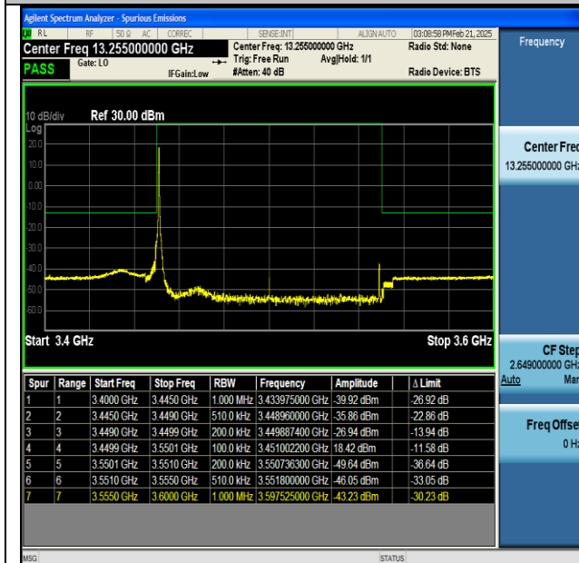
NTNV-n77(3450-3550)-PC2-30-100-L-CP-QPSK- Edge_1RB_Left-PASS
