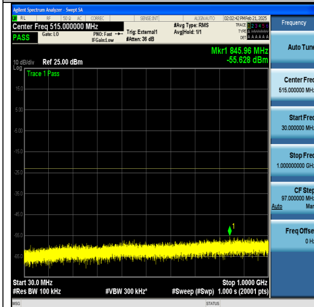
NTNV-n77(3450-3550)-PC2-30-100-H-DFT-BPSK- Edge_1RB_Left-30-1000-PASS
