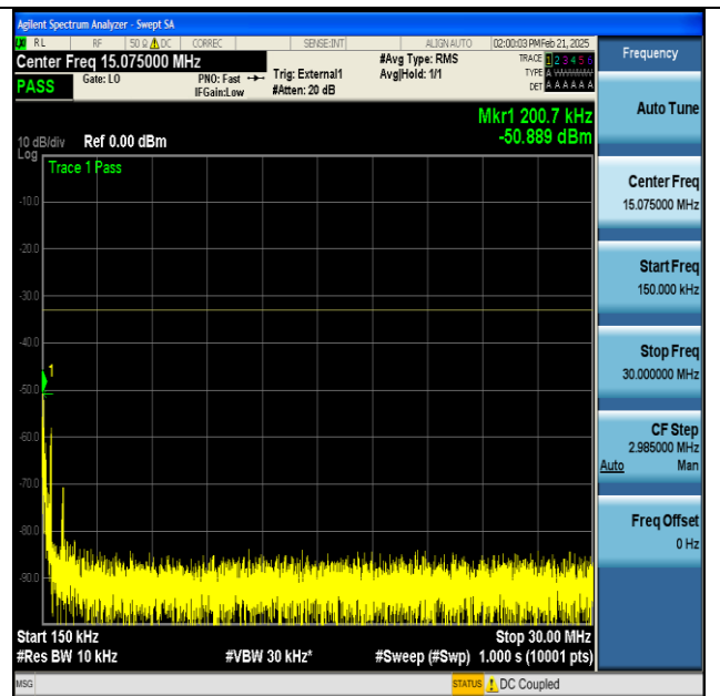
NTNV-n77(3450-3550)-PC2-30-100-M-CP-QPSK- Edge_1RB_Left-0.15-30-PASS
