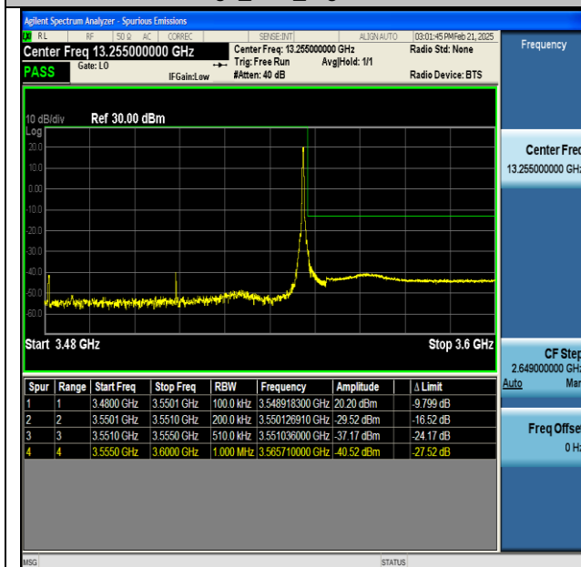
NTNV-n77(3450-3550)-PC2-30-70-H-CP-QPSK- Edge_1RB_Right-PASS
