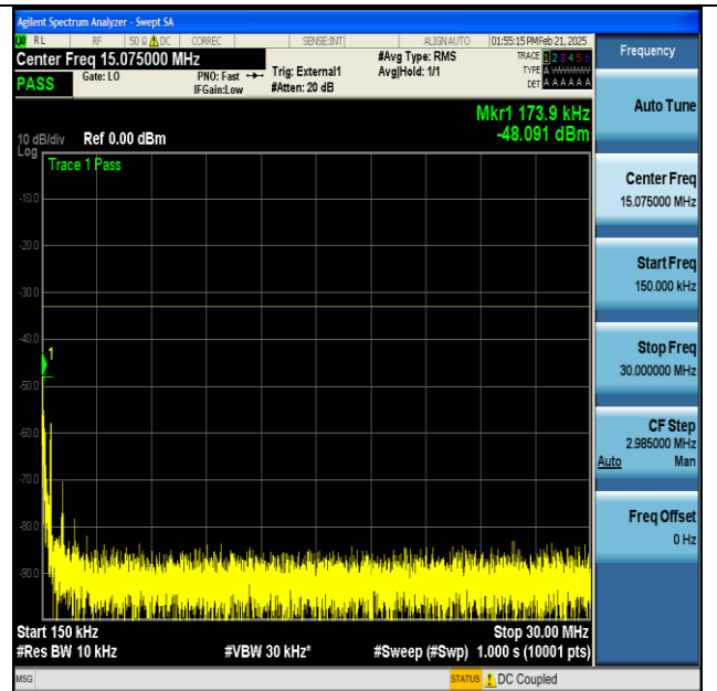
NTNV-n77(3450-3550)-PC2-30-100-L-CP-QPSK- Edge_1RB_Left-0.15-30-PASS
