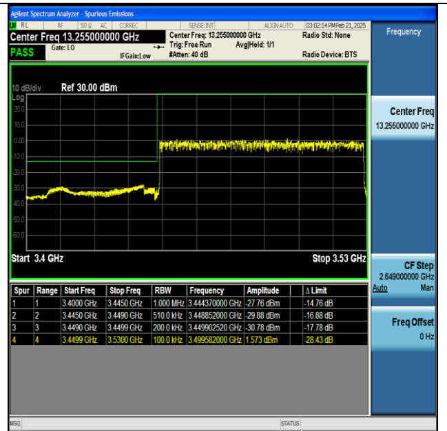
NTNV-n77(3450-3550)-PC2-30-80-L-DFT-BPSK- Outer_Full-PASS
