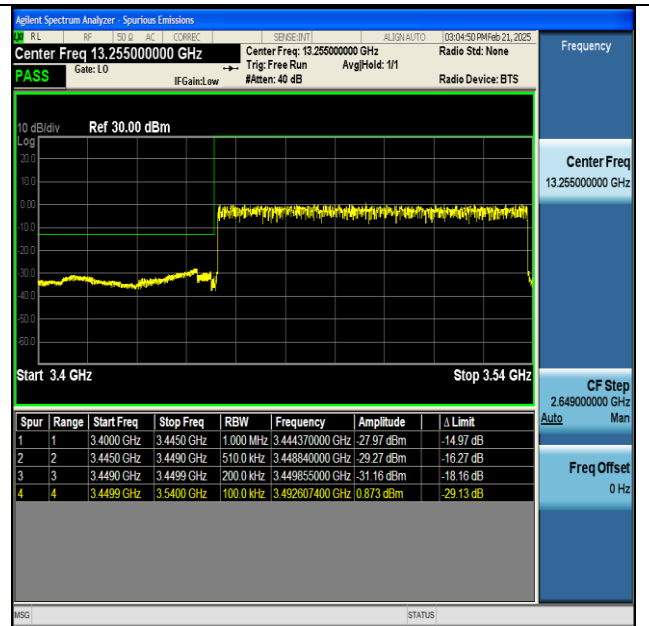
NTNV-n77(3450-3550)-PC2-30-90-L-DFT-BPSK- Outer_Full-PASS
