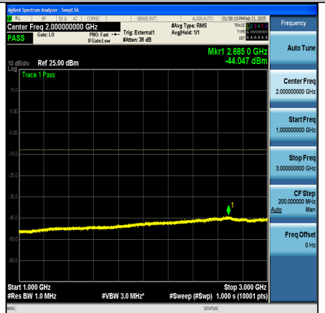
NTNV-n77(3450-3550)-PC2-30-100-M-DFT-BPSK- Edge_1RB_Left-1000-3000-PASS
