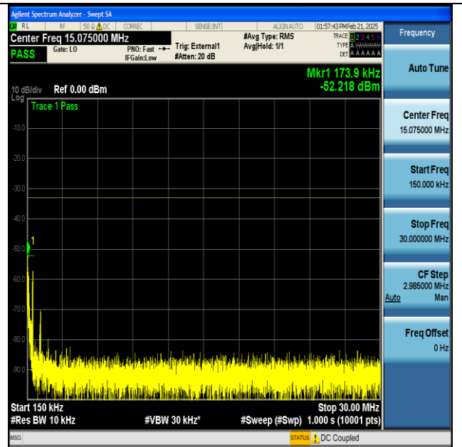
NTNV-n77(3450-3550)-PC2-30-100-M-DFT-BPSK- Edge_1RB_Left-0.15-30-PASS
