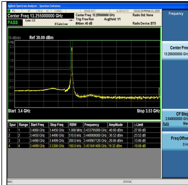
NTNV-n77(3450-3550)-PC2-30-80-L-DFT-BPSK- Edge_1RB_Left-PASS
