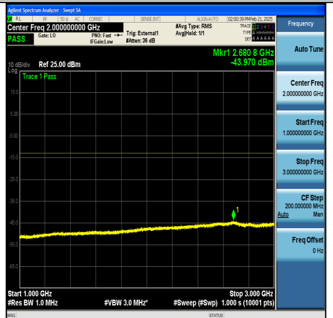
NTNV-n77(3450-3550)-PC2-30-100-M-CP-QPSK- Edge_1RB_Left-1000-3000-PASS
