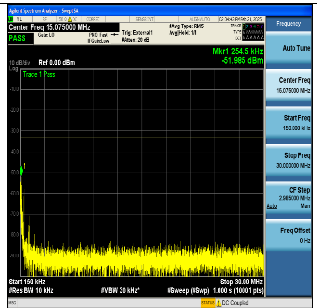
NTNV-n77(3450-3550)-PC2-30-100-H-CP-QPSK- Edge_1RB_Left-0.15-30-PASS
