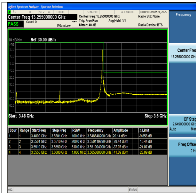
NTNV-n77(3450-3550)-PC2-30-70-H-DFT-BPSK- Edge_1RB_Right-PASS
