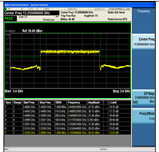
NTNV-n77(3450-3550)-PC2-30-100-H-DFT-BPSK- Outer_Full-PASS
