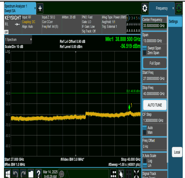
NTNV-n77(3450-3550)-PC2-30-100-M-CP-QPSK- Edge_1RB_Left-27000-40000-PASS
