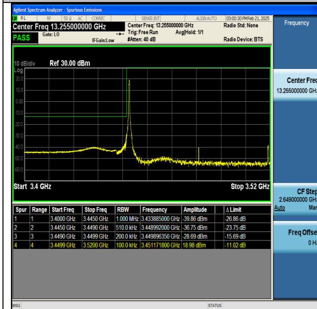
NTNV-n77(3450-3550)-PC2-30-70-L-CP-QPSK- Edge_1RB_Left-PASS
