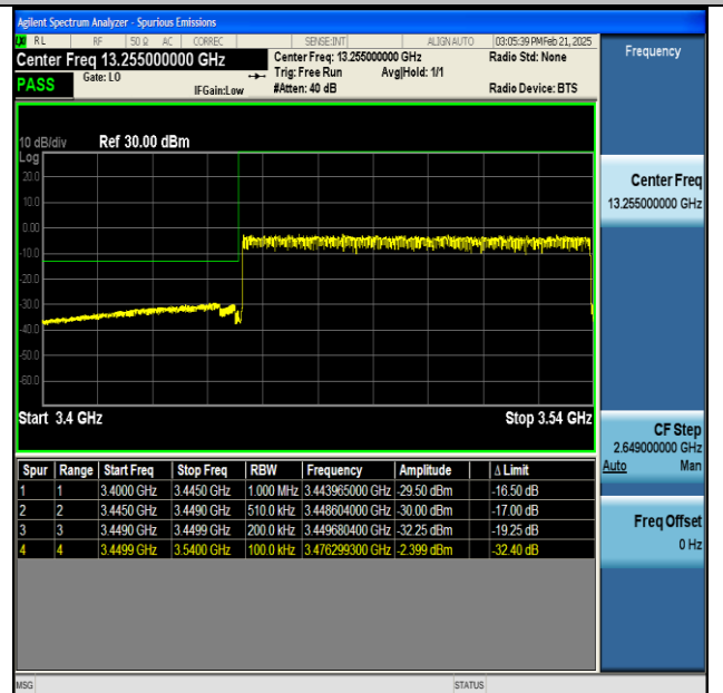
NTNV-n77(3450-3550)-PC2-30-90-L-CP-QPSK- Outer_Full-PASS
