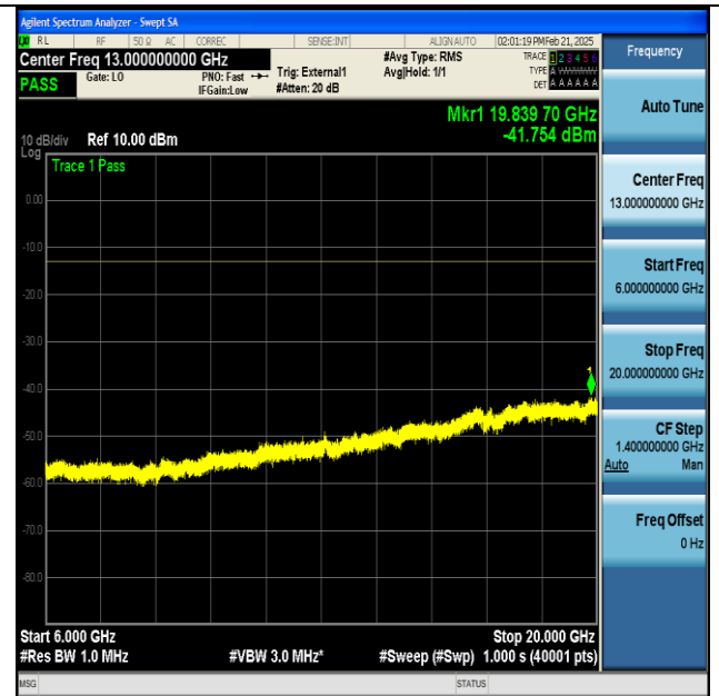
NTNV-n77(3450-3550)-PC2-30-100-M-CP-QPSK- Edge_1RB_Left-6000-20000-PASS
