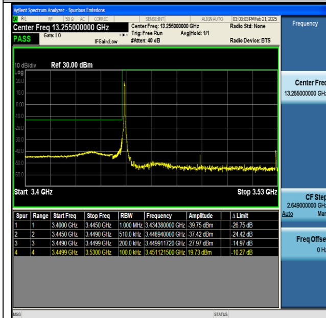
NTNV-n77(3450-3550)-PC2-30-80-L-CP-QPSK- Edge_1RB_Left-PASS
