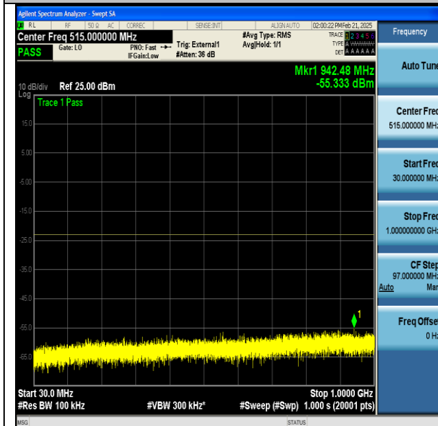
NTNV-n77(3450-3550)-PC2-30-100-M-CP-QPSK- Edge_1RB_Left-30-1000-PASS
