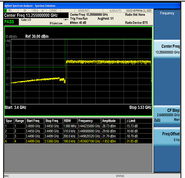
NTNV-n77(3450-3550)-PC2-30-80-L-CP-QPSK- Outer_Full-PASS
