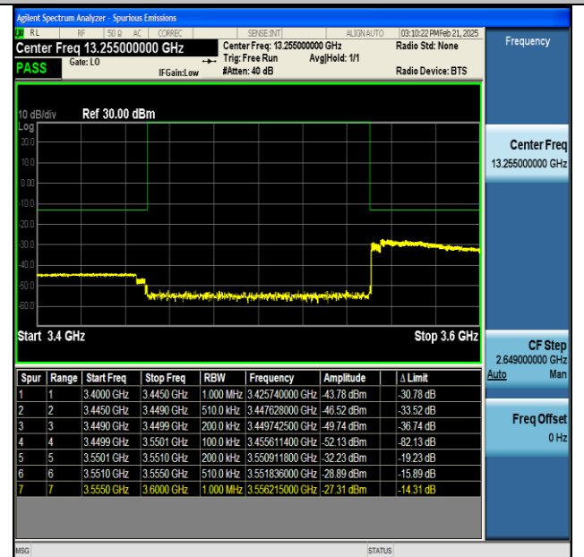
NTNV-n77(3450-3550)-PC2-30-100-H-CP-QPSK- Outer_Full-PASS
