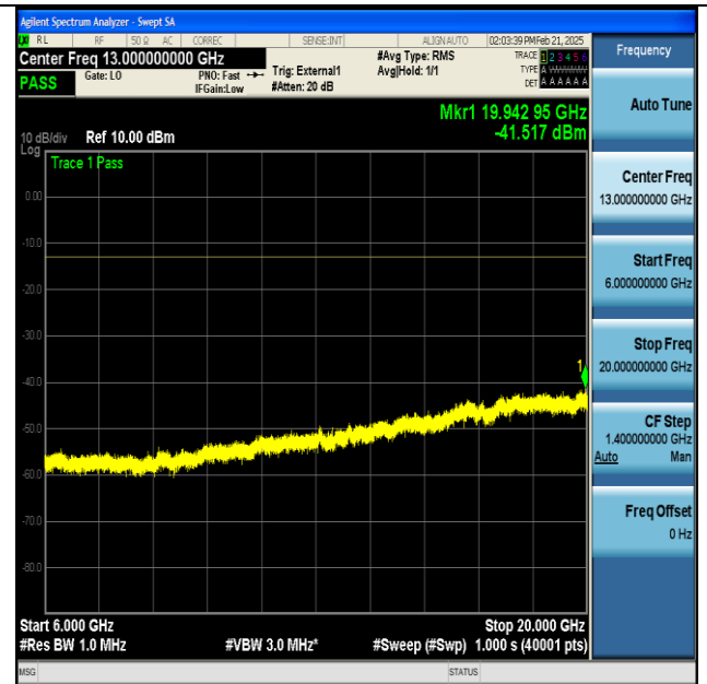
NTNV-n77(3450-3550)-PC2-30-100-H-DFT-BPSK- Edge_1RB_Left-6000-20000-PASS
