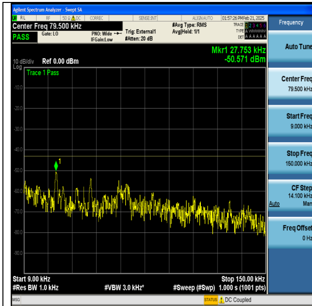
NTNV-n77(3450-3550)-PC2-30-100-M-DFT-BPSK- Edge_1RB_Left-0.009-0.15-PASS
