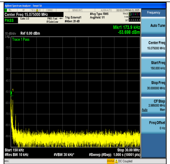
NTNV-n77(3450-3550)-PC2-30-100-H-DFT-BPSK- Edge_1RB_Left-0.15-30-PASS
