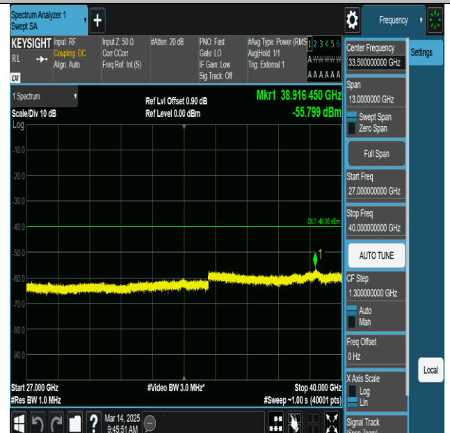
NTNV-n77(3450-3550)-PC2-30-100-H-DFT-BPSK- Edge_1RB_Left-27000-40000-PASS
