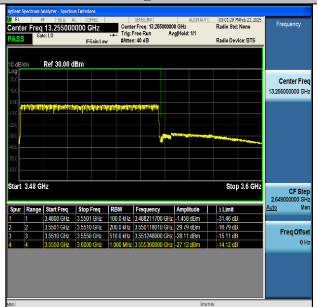
NTNV-n77(3450-3550)-PC2-30-70-H-CP-QPSK- Outer_Full-PASS
