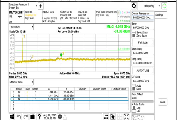
Band12 5MHz Chain0 701.5MHz NBI 0 QPSK 1 0
