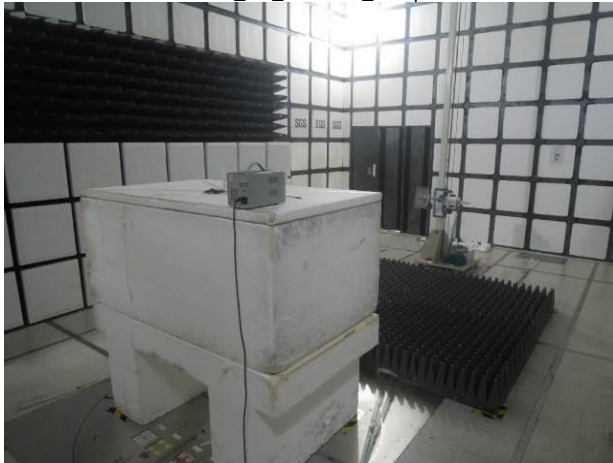
CAT_M1_Radiated_Setup
