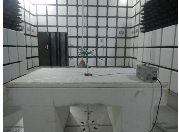
CAT_M1_Radiated_Setup
