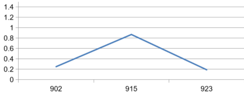
Peak Gain(dBi)
