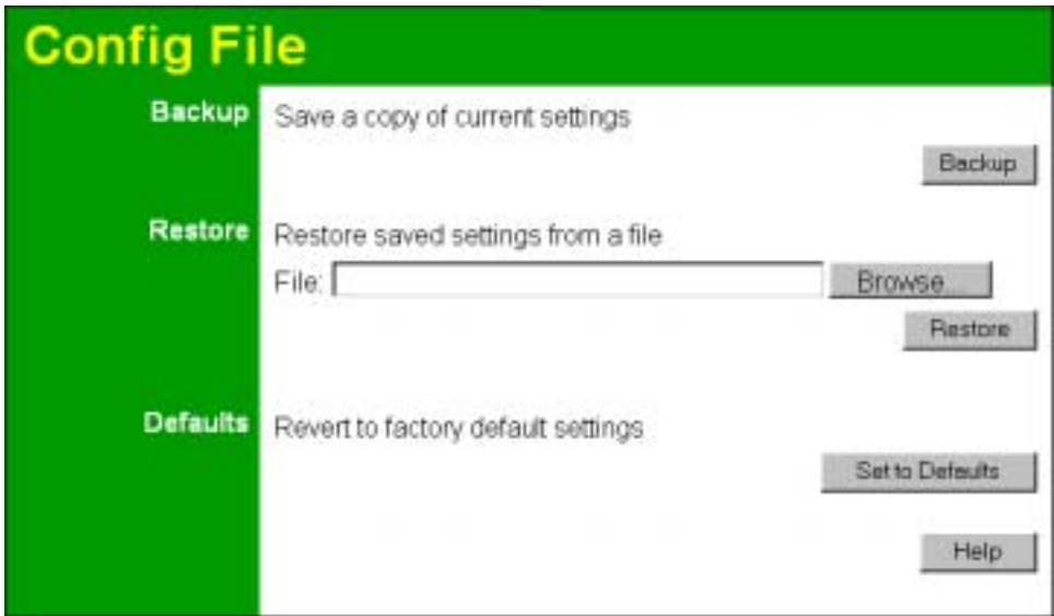
Figure 61: Config File Screen
