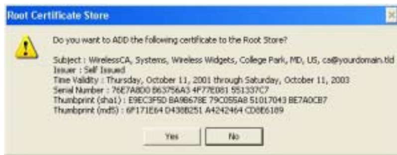
Figure 50: Root Certificate Screen
