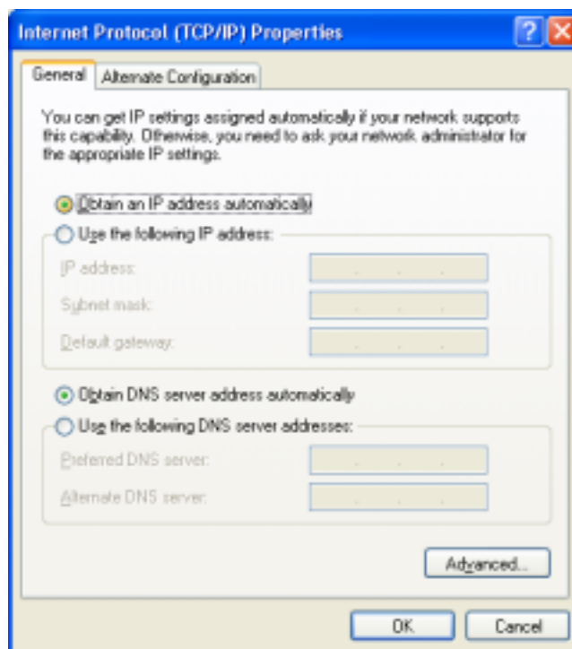
Figure 72: TCP/IP Properties (Windows XP)
