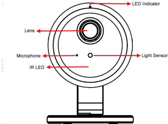
Figure 1: Front Panel
