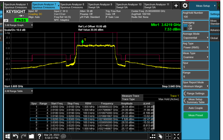
FULL CH 55990 (3625 MHz)
