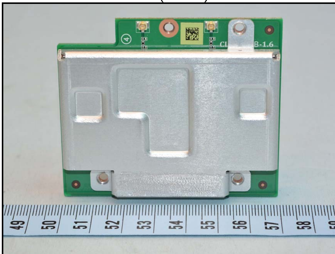
RF 3(Band 4)
