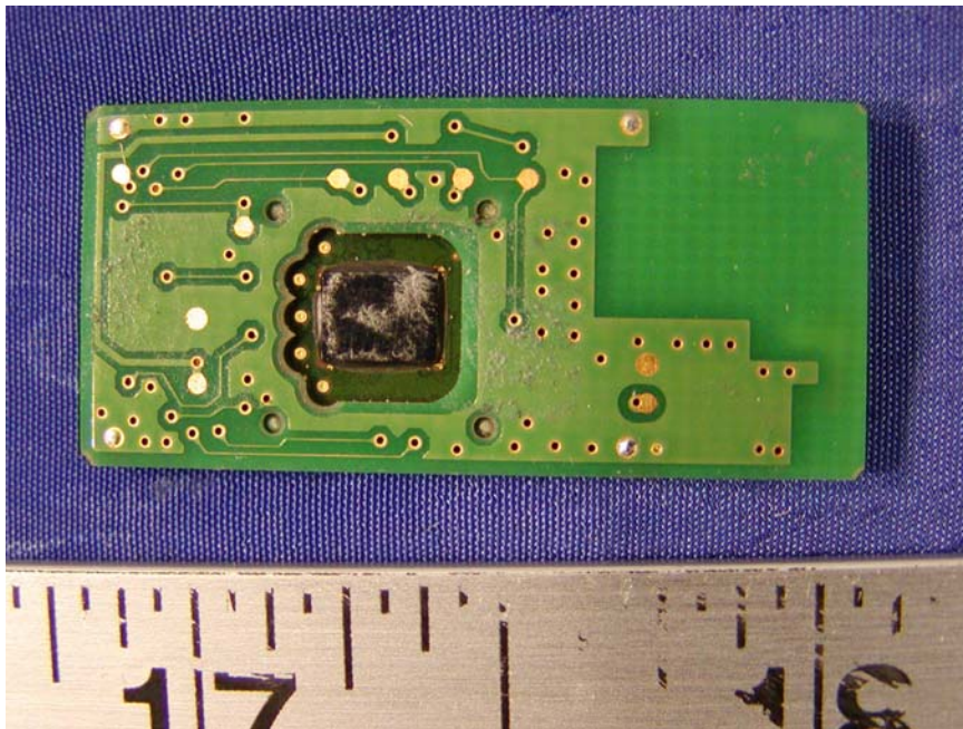
EUT – PCB Solder View
