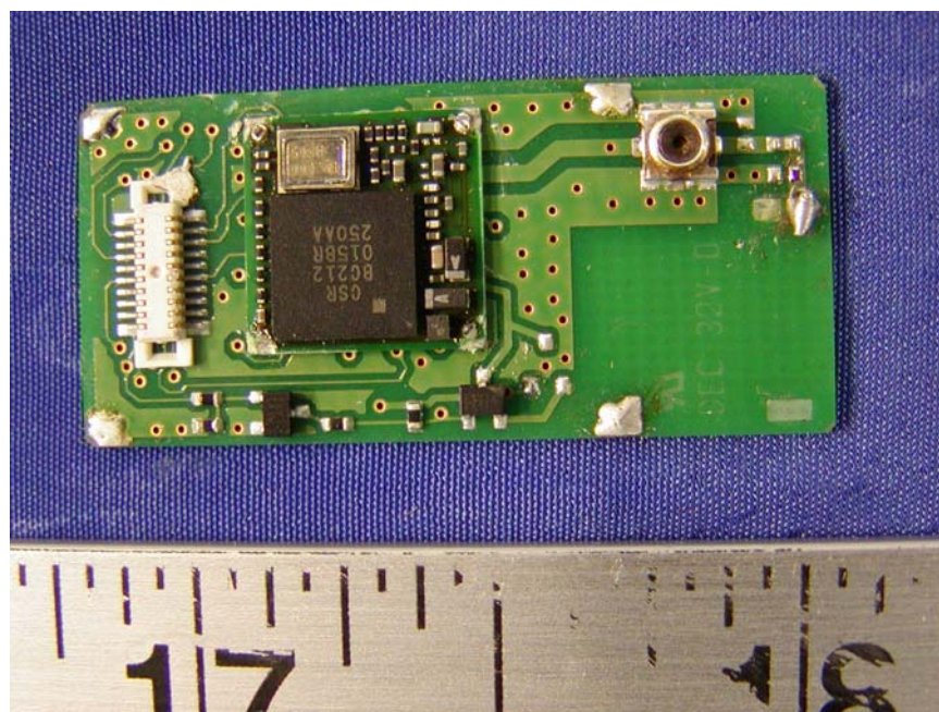
EUT – PCB Top View without Shield
