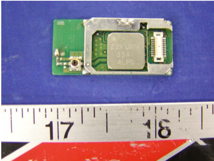
EUT – PCB Top View with Shield
