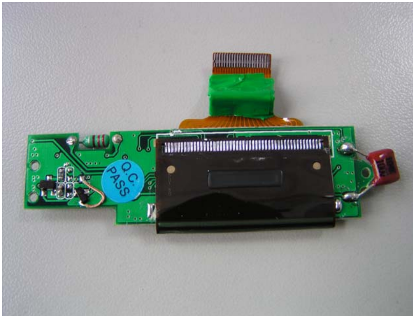
EUT – PCB View (4)
