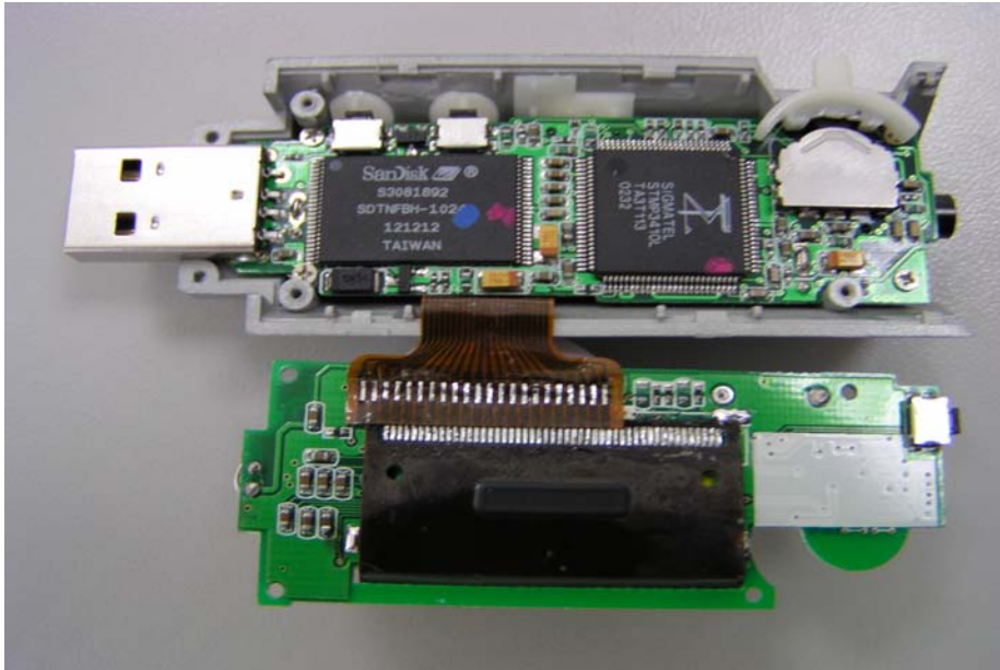
EUT -PCB View (1)
