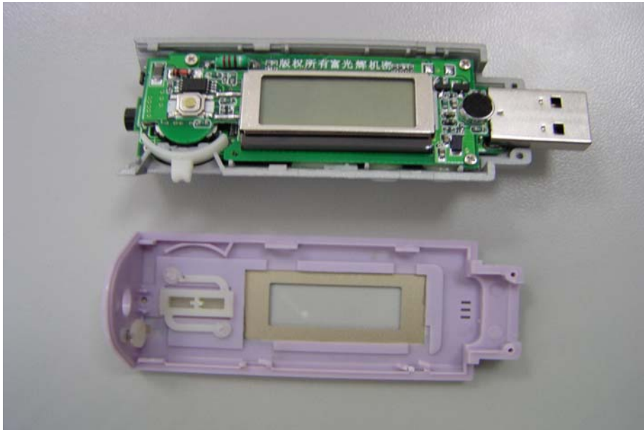
EUT – Inside view (1)
