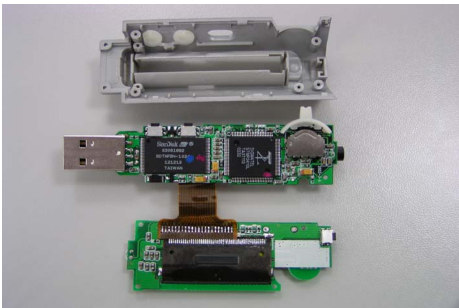
EUT - Inside View (2)
