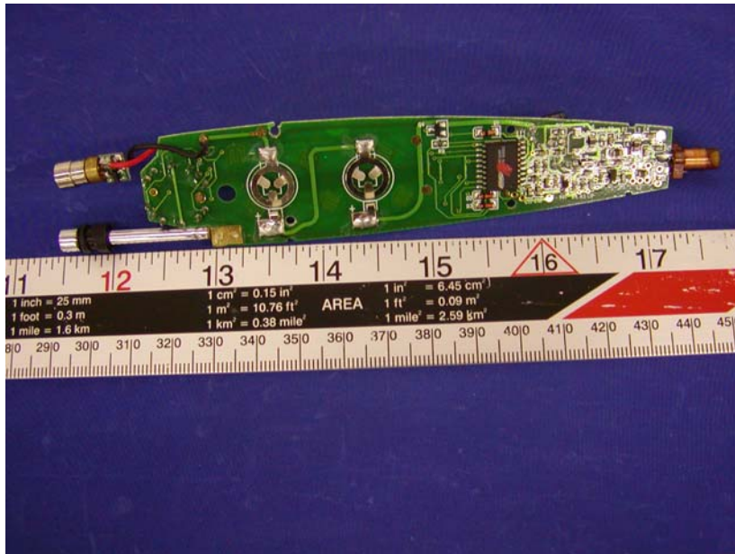
Transmitter PCB view (2)
