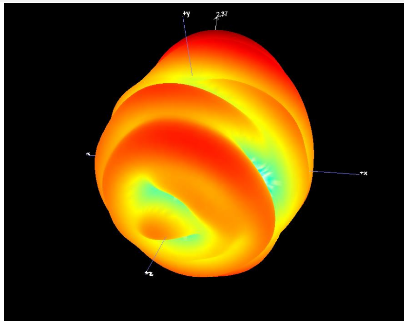
B1.2 3D Pattern for 5800MHz
