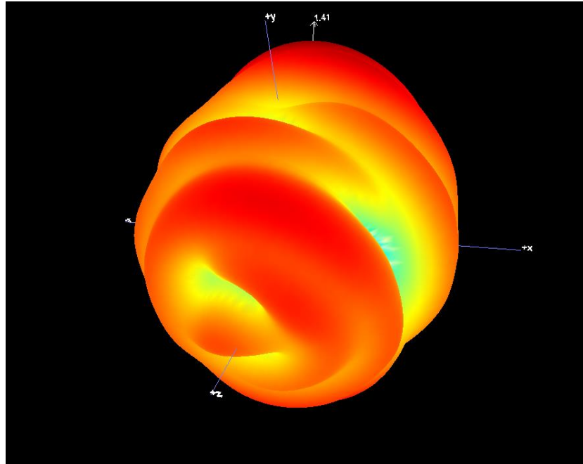
B1.1 3D Pattern for 5725MHz
