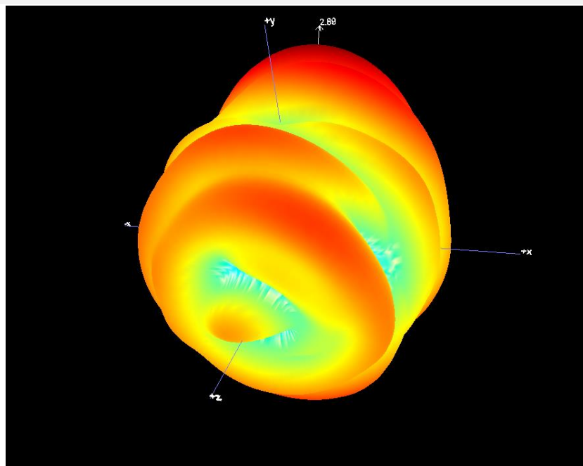
B1.3 3D Pattern for 5850MHz
