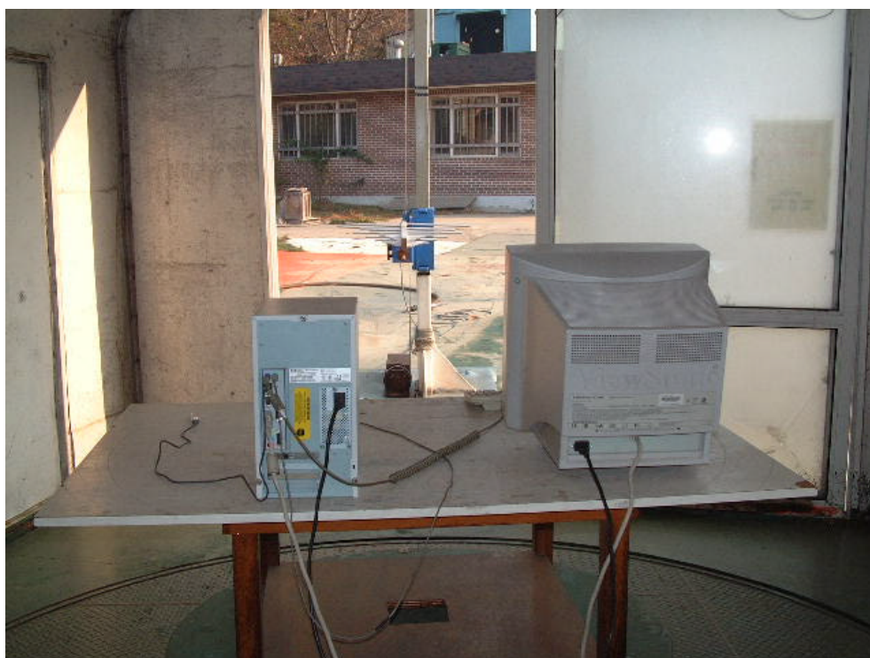
RADIATED EMISSION SETUP PHOTOGRAPH - REAR VIEW ( 300 - 1000 MHz )
