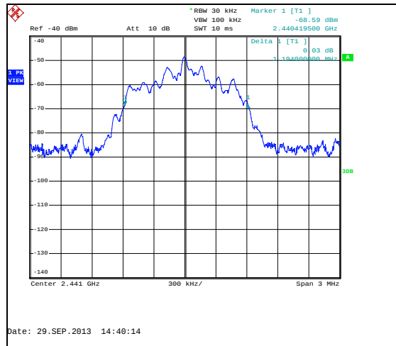
Figure 7.3.2-14: 20dB BW Mid CH (8DPSK - 3Mbps)
