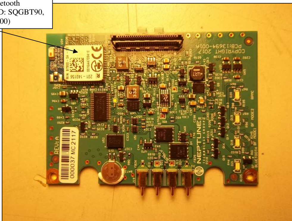
Figure 8: Internal Photo
