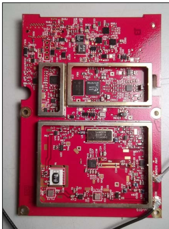
Figure 18: Internal Photo
