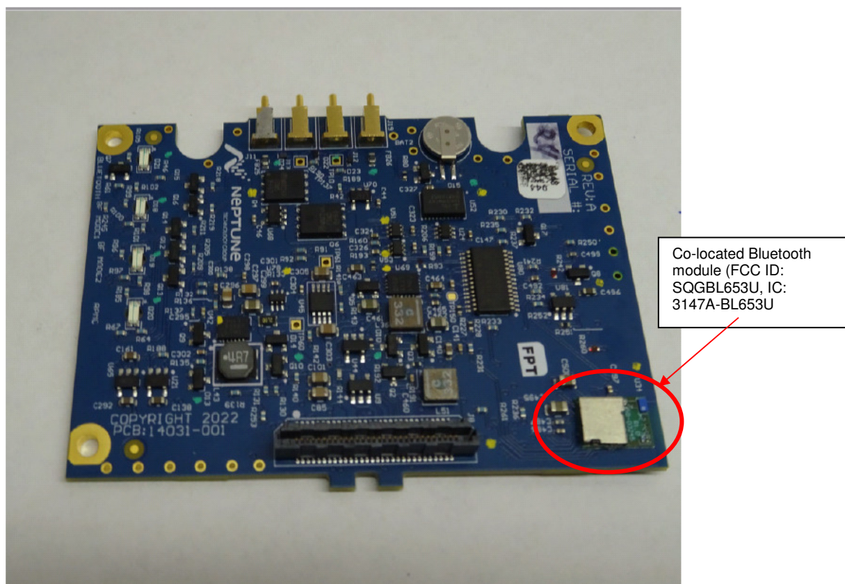
Figure 1. LVPS Board top
