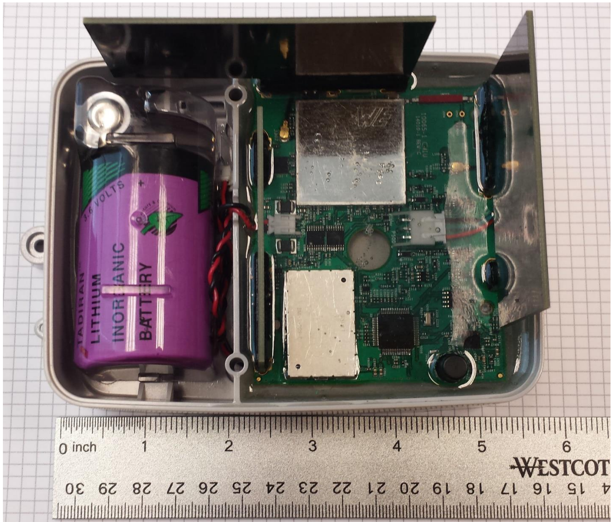
Figure 3: CMIU Internal Top (potted)
