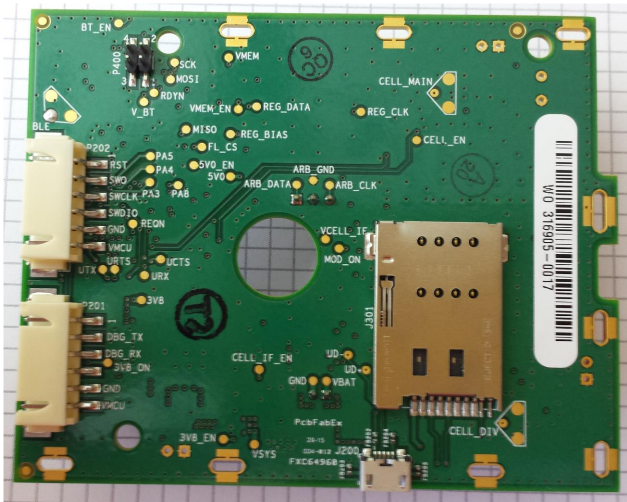
Figure 5: Main PCB, Bottom/Connector Side
