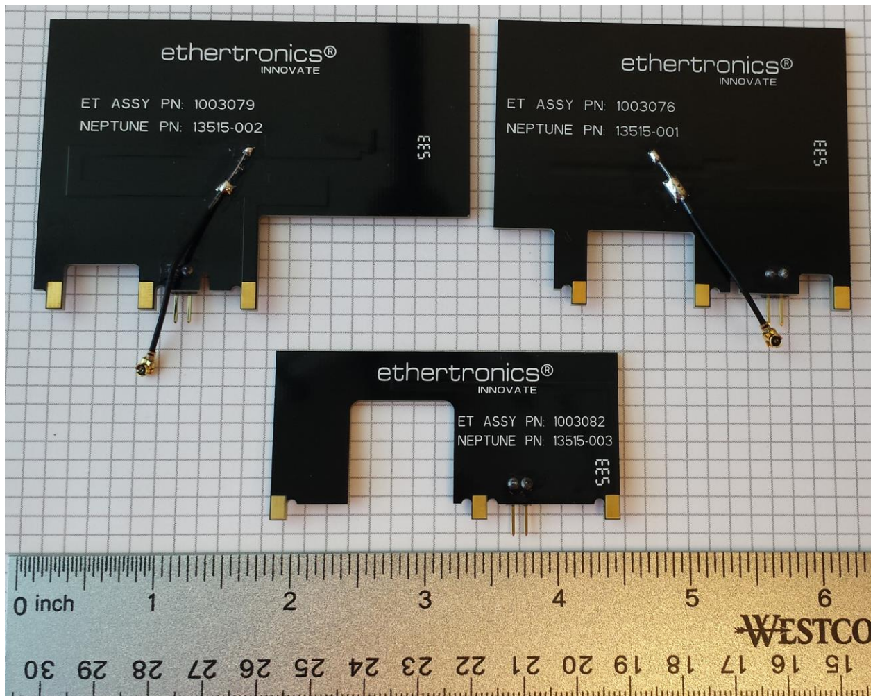
Figure 6: Antenna PCBs
