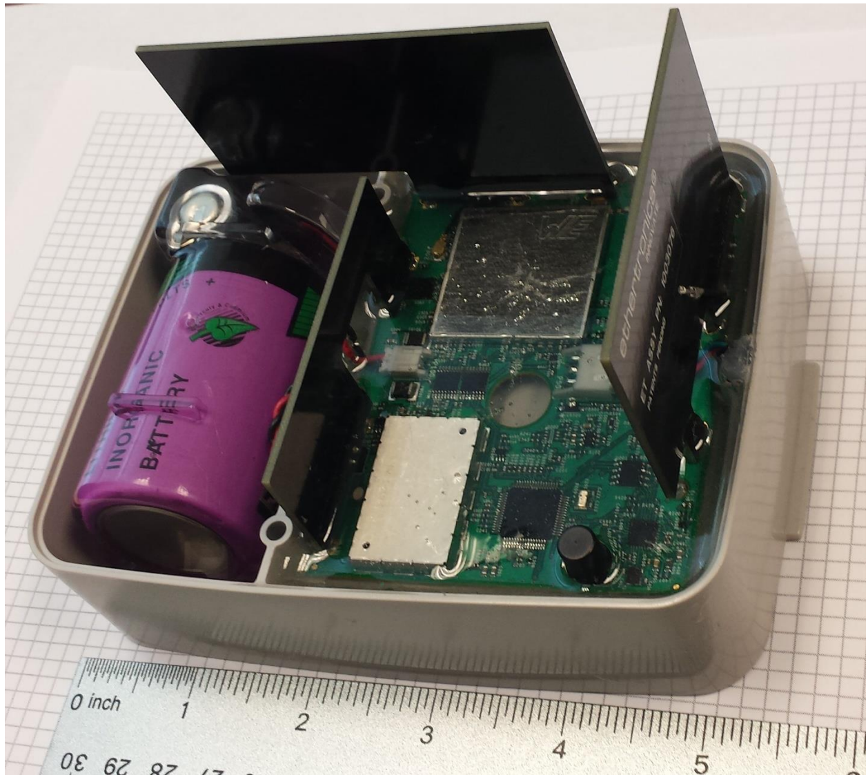
Figure 3: CMIU Internal Profile (potted)
