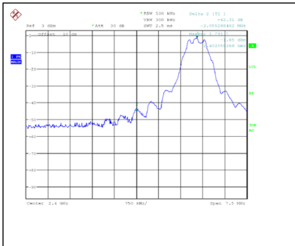
Figure 7.5.1.2-4: Lower Band-edge - LCH
