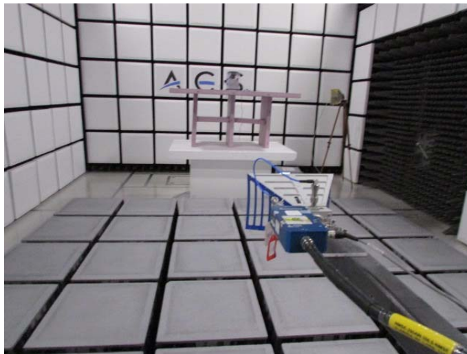
Figure 1: Radiated Spurious Emissions – Front View – Above 1GHz
