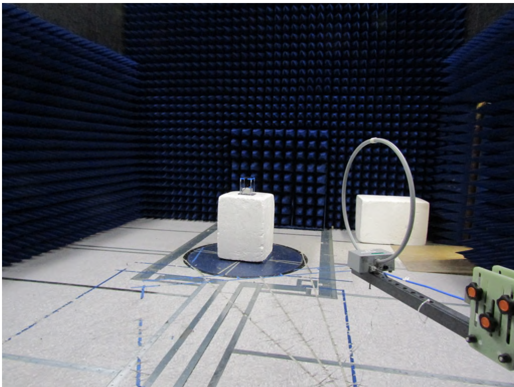
Figure 8: Equipment Under Test – Radiated Emissions <30MHz (Pit Mount)
