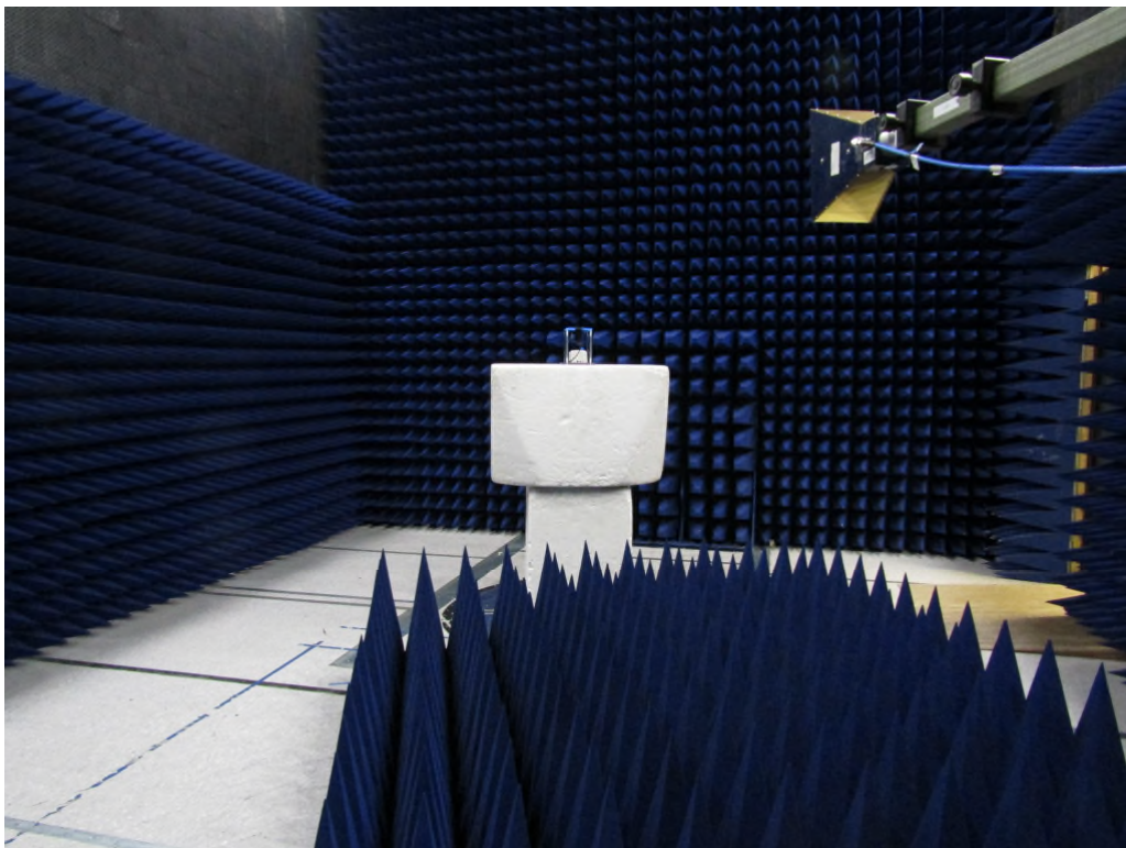
Figure 10: Equipment Under Test – Radiated Emissions >1GHz (Pit Mount)
