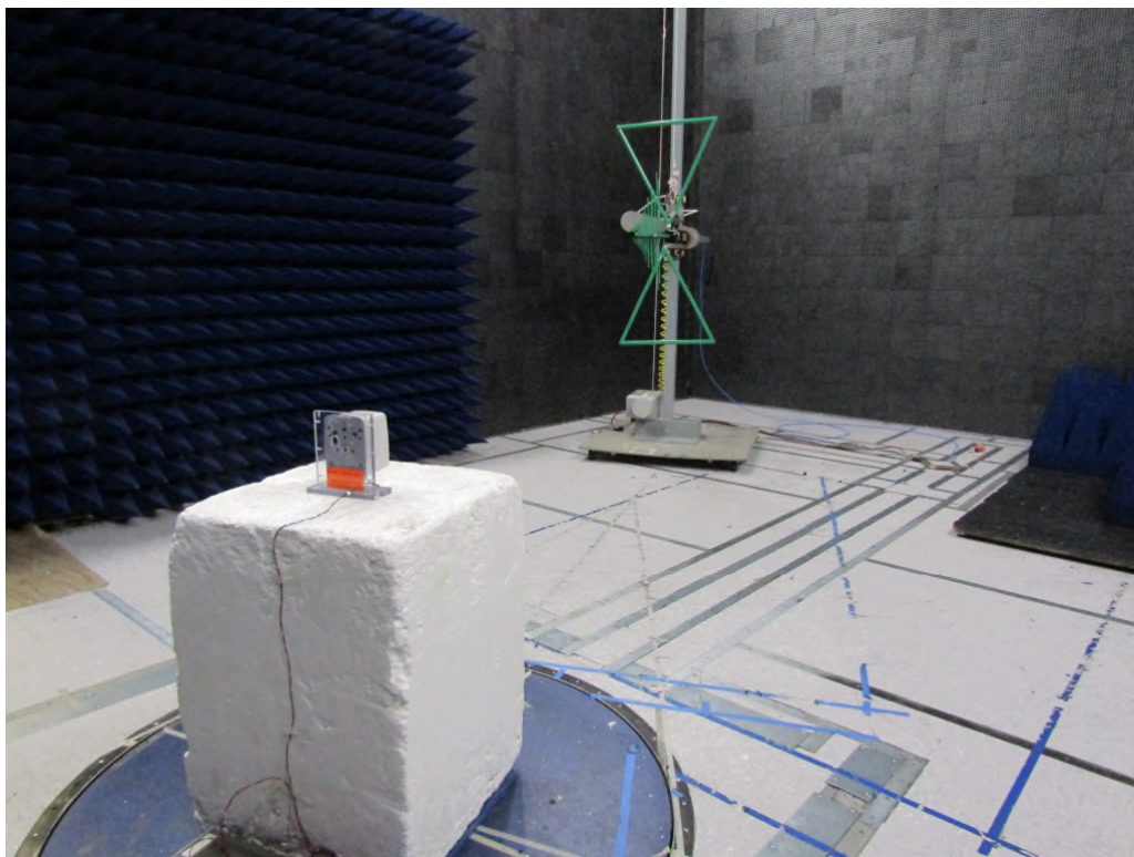
Figure 5: Equipment Under Test – Radiated Emissions <1GHz (Wall Mount)
