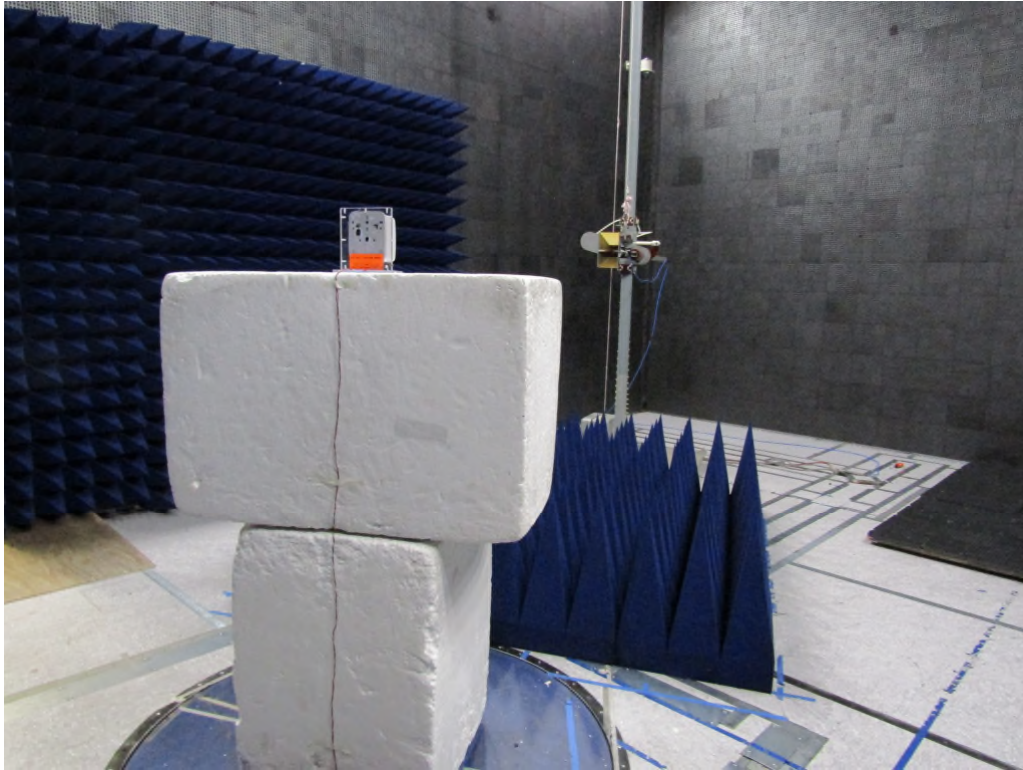
Figure 7: Equipment Under Test – Radiated Emissions >1GHz (Wall Mount)
