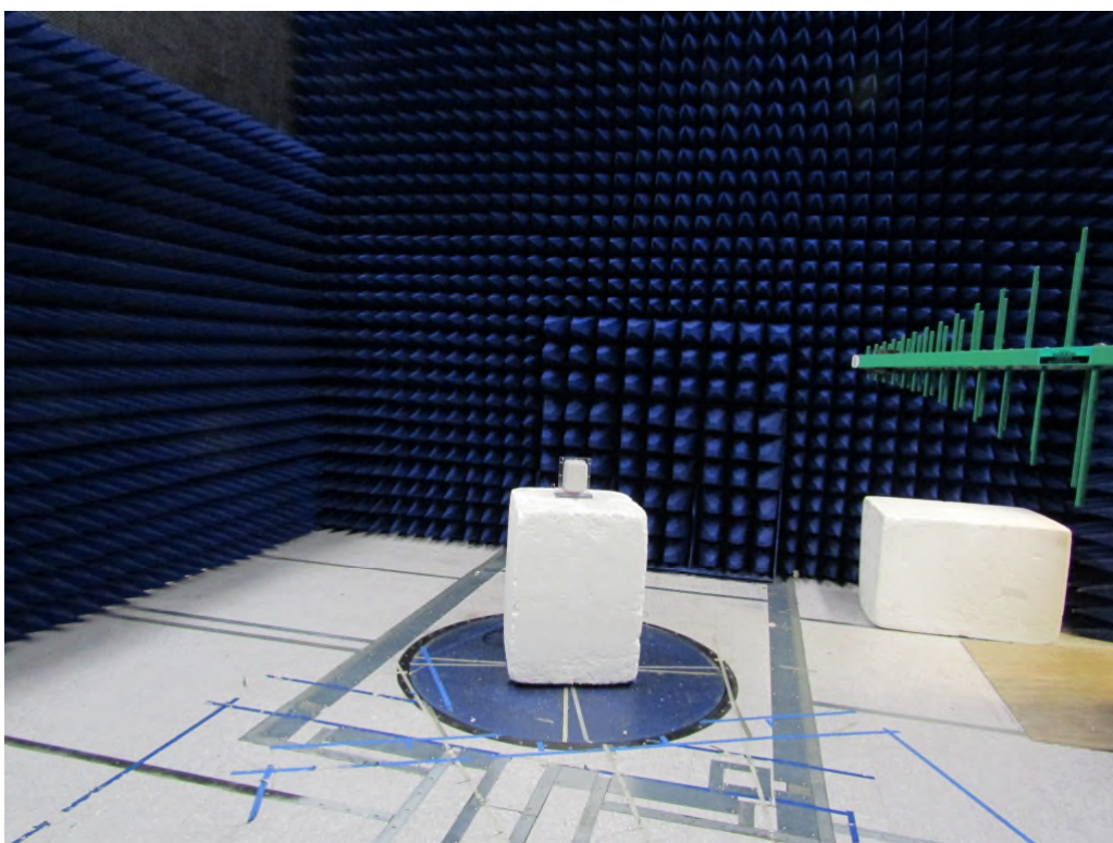
Figure 4: Equipment Under Test – Radiated Emissions <1GHz (Wall Mount)
