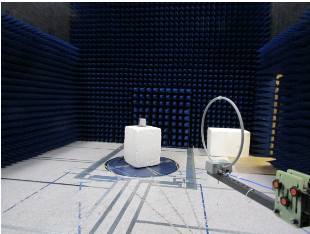
Figure 3: Equipment Under Test – Radiated Emissions <30MHz (Wall Mount)
