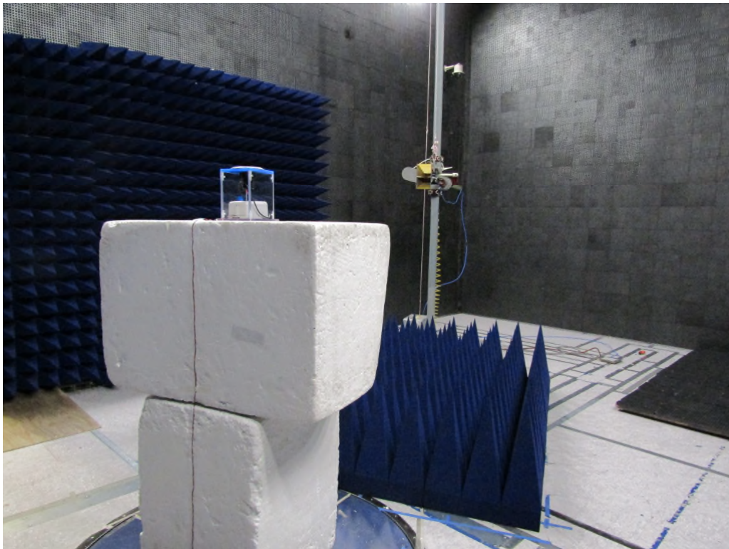
Figure 11: Equipment Under Test – Radiated Emissions >1GHz (Pit Mount)
