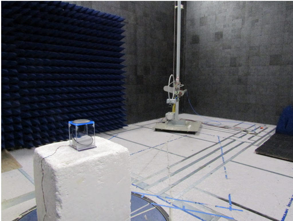
Figure 9: Equipment Under Test – Radiated Emissions <30MHz (Pit Mount)
