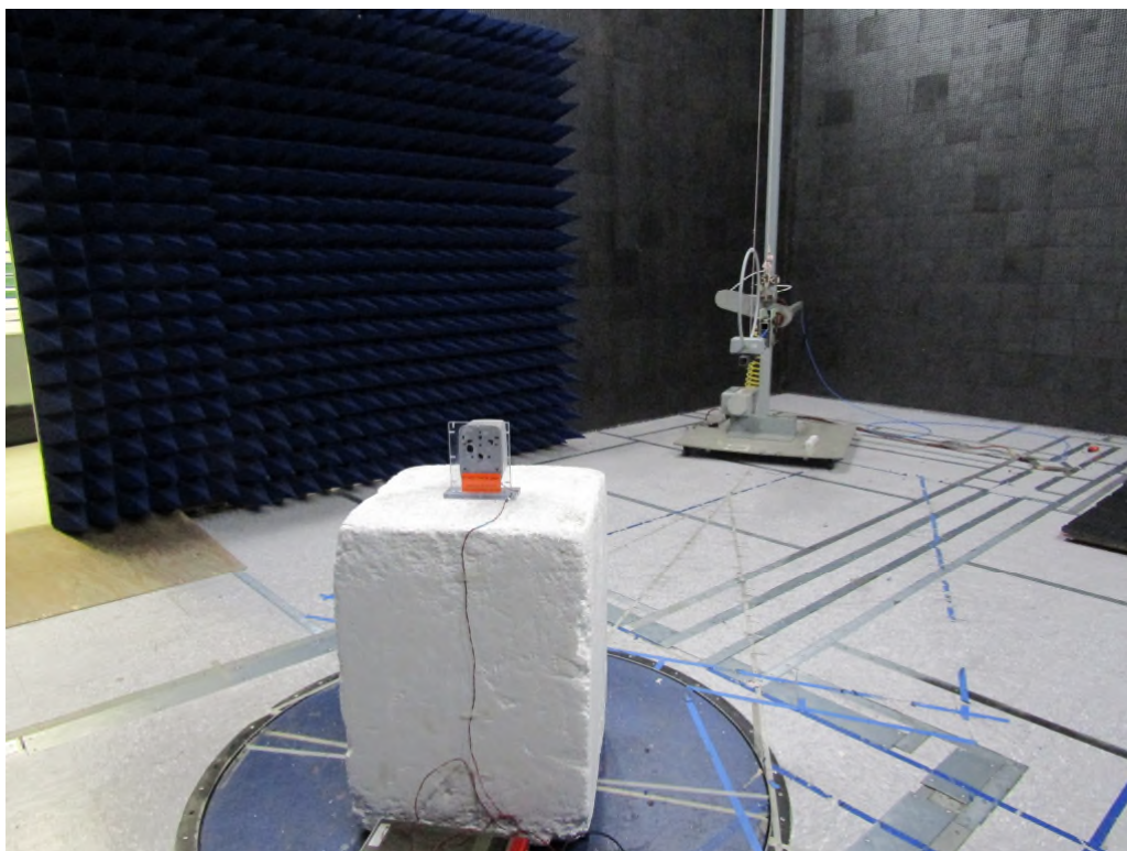
Figure 2: Equipment Under Test – Radiated Emissions <30MHz (Wall Mount)
