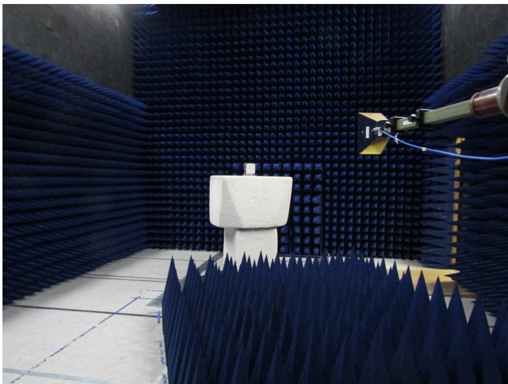
Figure 6: Equipment Under Test – Radiated Emissions >1GHz (Wall Mount)
