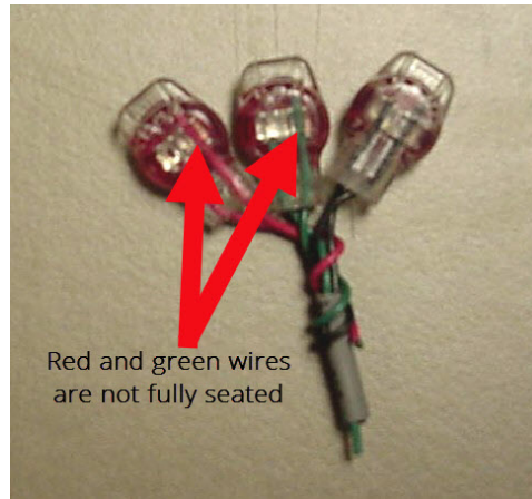
Figure 39 – Improper Connections
