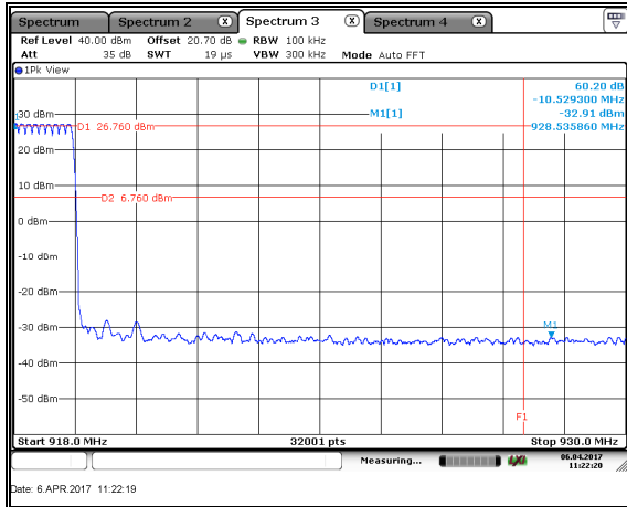
Figure 7.4.1.2-6: Upper Band-Edge Hopping - GFSK
