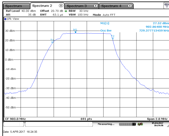
Figure 7.2.2-4: 99% OBW – LCH
