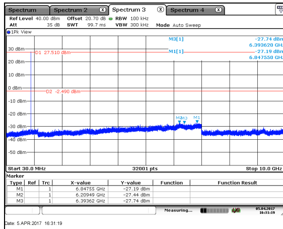
Figure 7.4.1.2-1: RF Conducted Emissions – LCH
