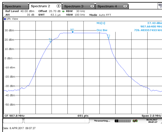
Figure 7.2.2-5: 99% OBW – MCH
