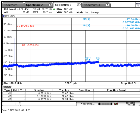
Figure 7.4.1.2-2: RF Conducted Emissions – MCH
