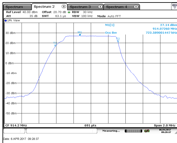
Figure 7.2.2-6: 99% OBW – HCH
