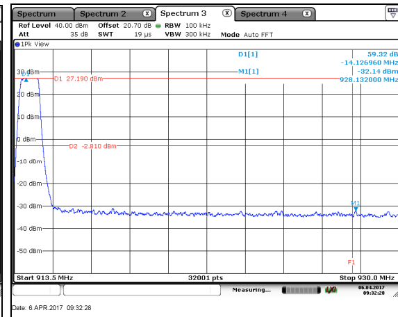
Figure 7.4.1.2-5: Upper Band-edge
