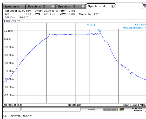
Figure 7.5.2-1: PSD – LCH
