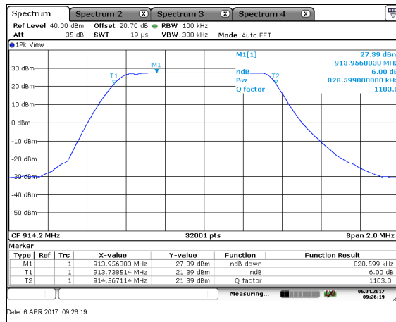
Figure 7.2.2-3: 6dB BW – HCH
