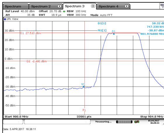
Figure 7.4.1.2-4: Lower Band-edge
