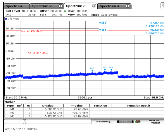
Figure 7.4.1.2-3: RF Conducted Emissions – HCH
