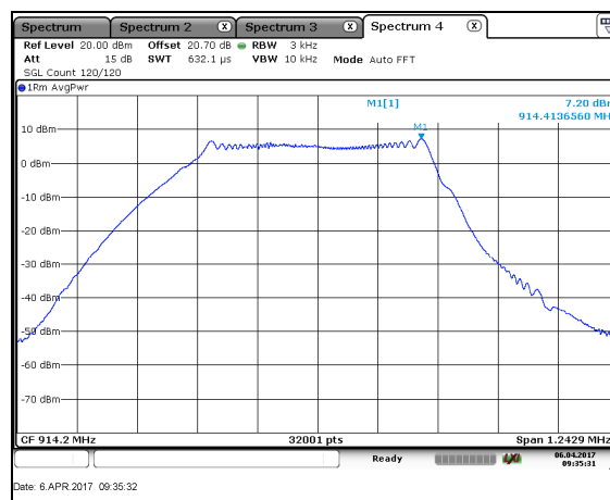
Figure 7.5.2-3: PSD – HCH
