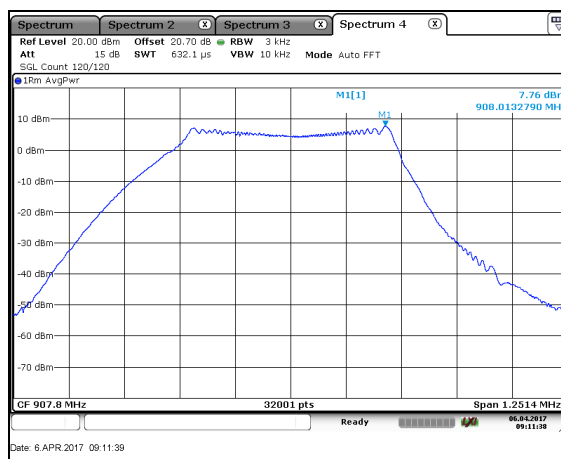
Figure 7.5.2-2: PSD – MCH
