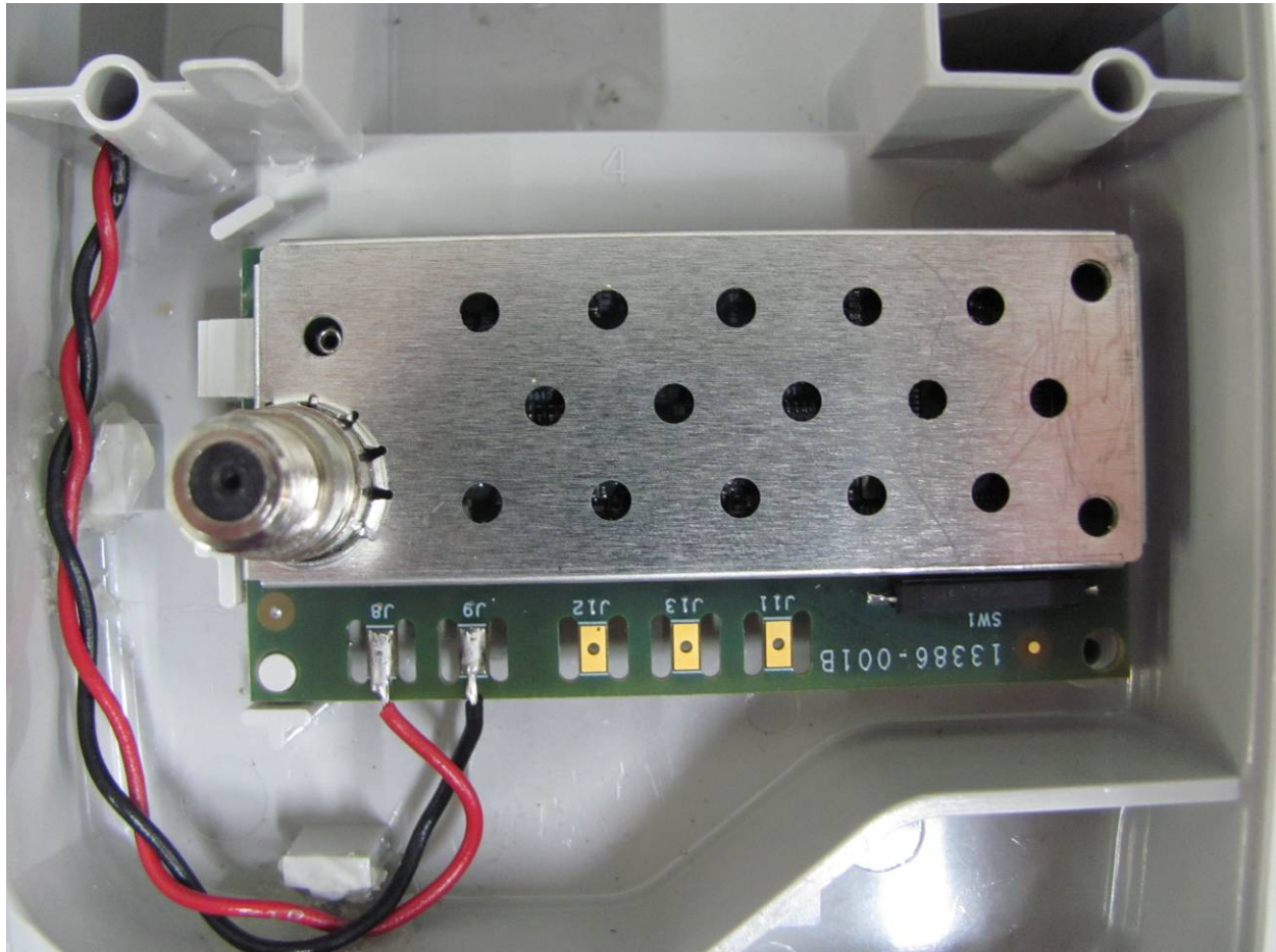
Figure 2. Close up of Module in Test Fixture, with Shield
