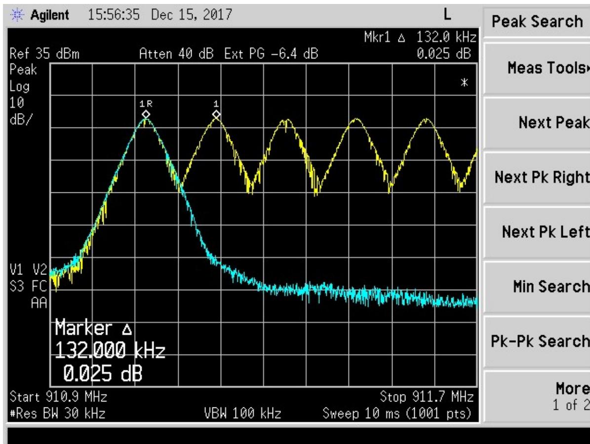
Figure 20. Channel Separation
