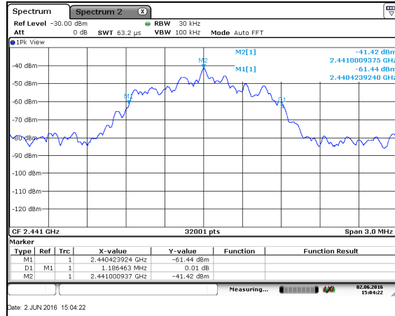
Figure 7.3.2-14: 20dB BW Mid CH (8DPSK - 3Mbps)
