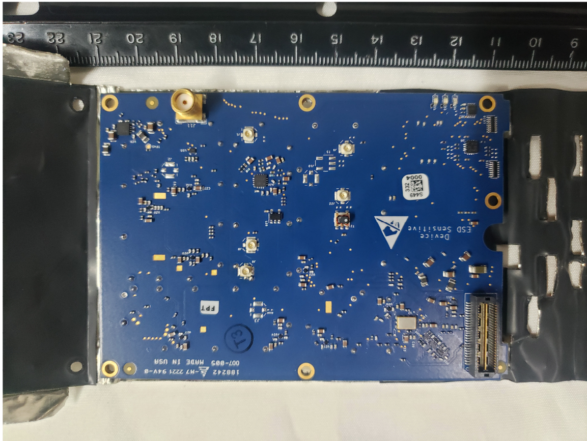
Figure 2. RF Board bottom
