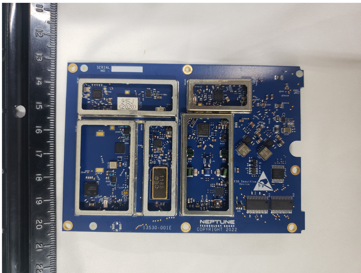
Figure 1. RF Board top
