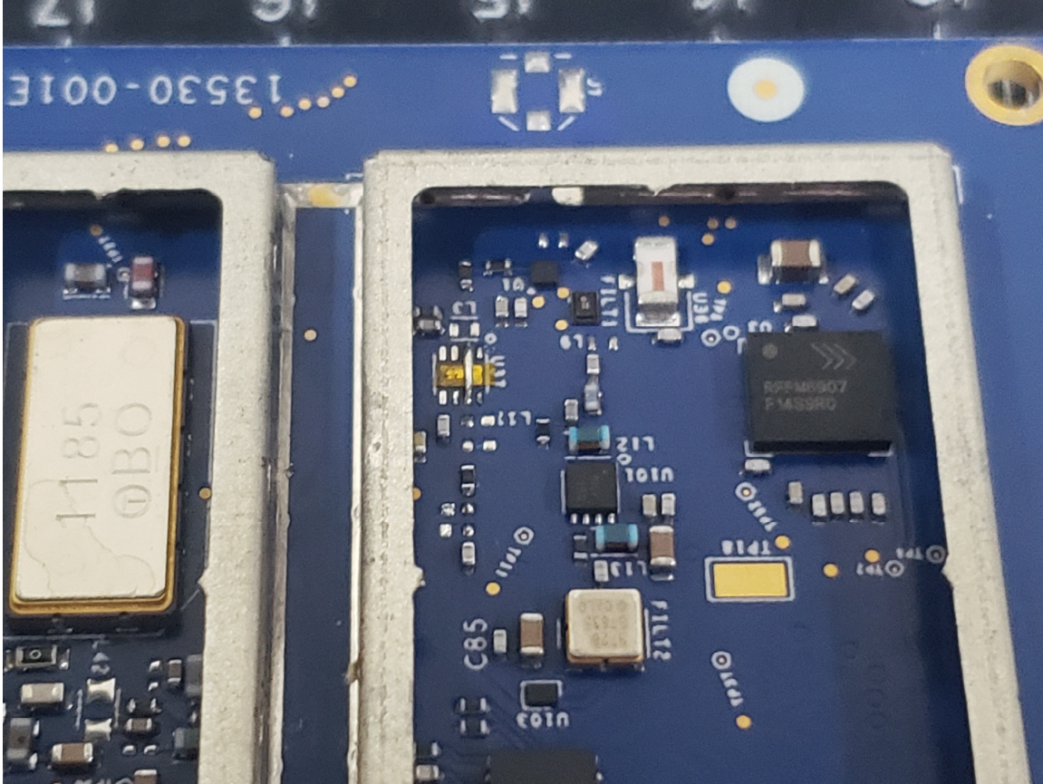
Figure 3. Close up of changes to board
