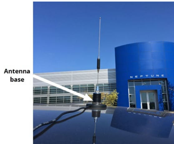
Figure 3.10 Antenna Installation
