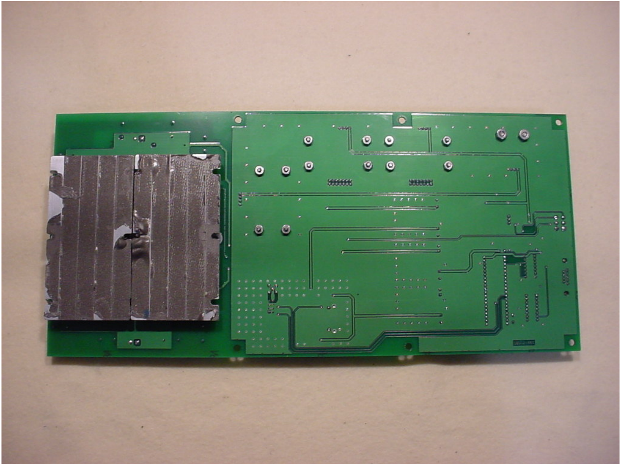
Figure 5: Internal – PCB Bottom
