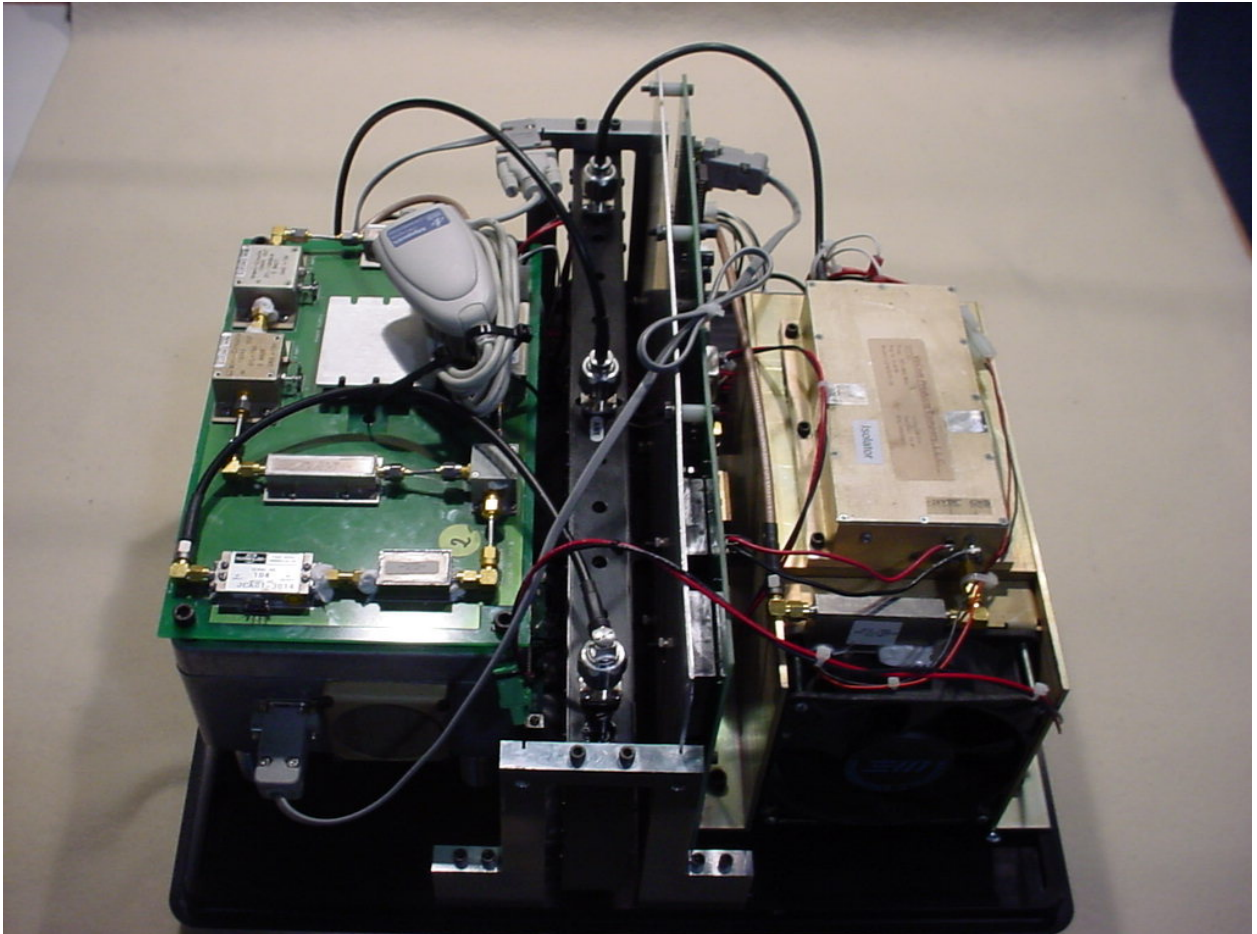
Figure 1: Internal – Assembled Top
