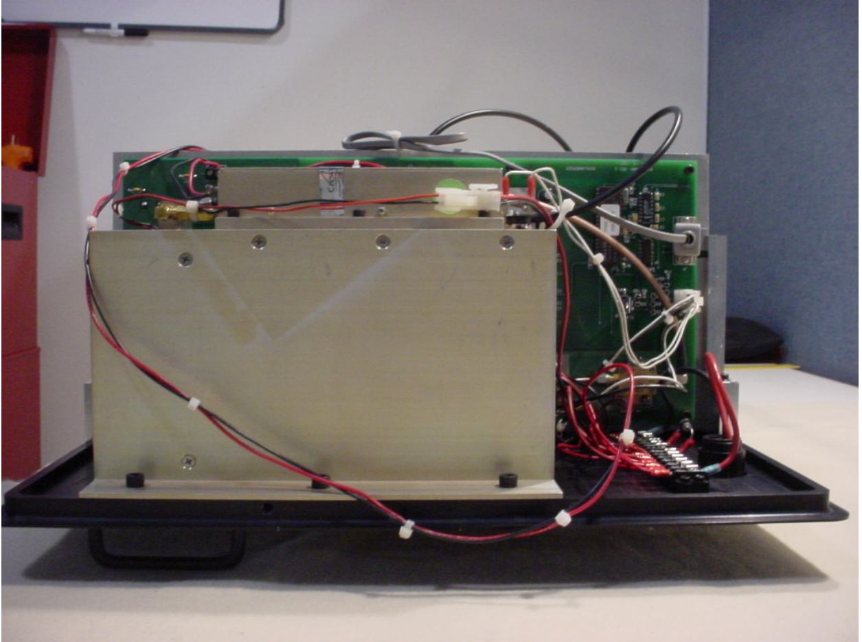
Figure 2: Internal – Assembled Side
