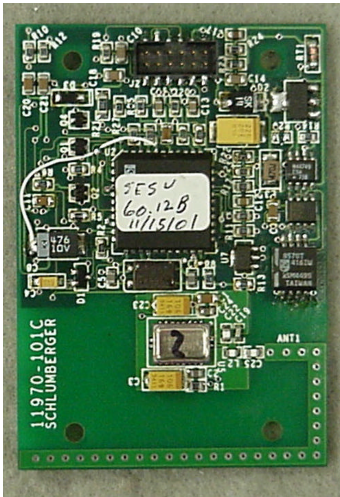
Photo 14, EUT, Top Side of Transmitter Board
