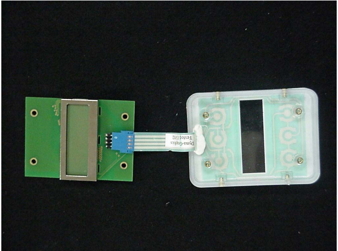
Photo 8. EUT, Top Side of Display Board and Button Components
