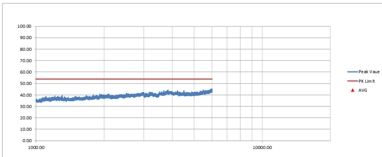
Figure 5. Radiated Emissions above 1 GHz, Vertical Polarity
