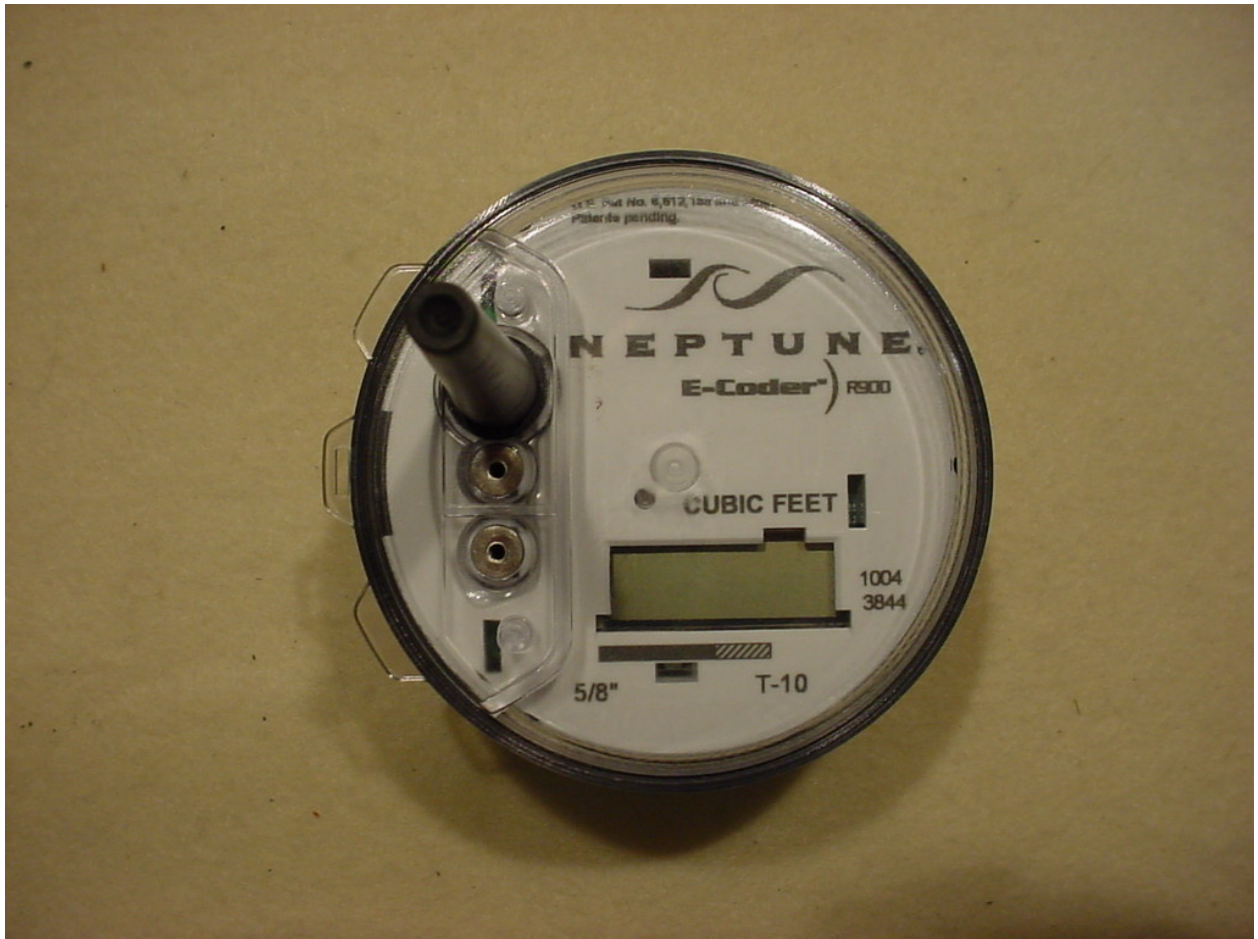
Figure 2: Top View
