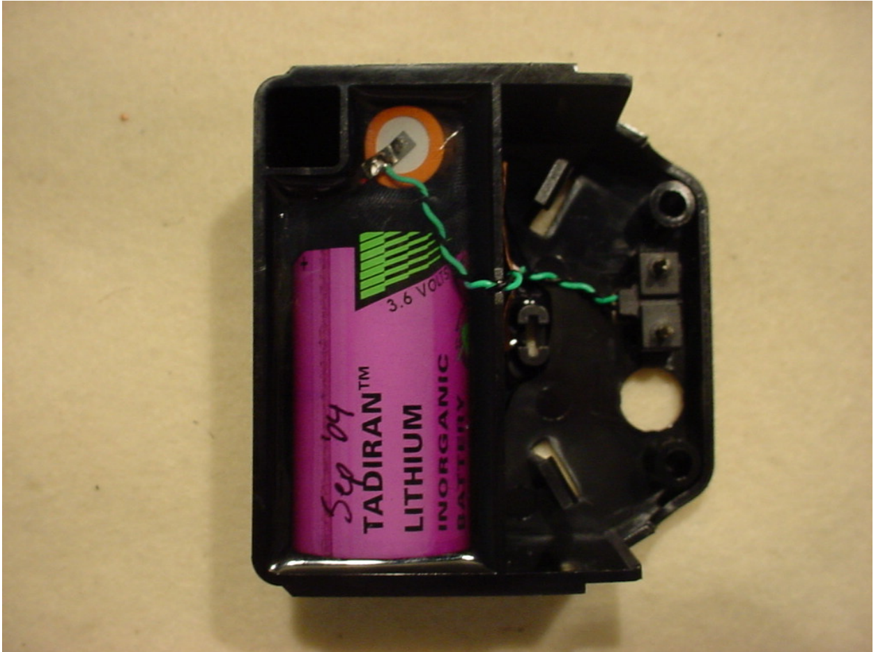
Figure 4: Bottom View Battery
