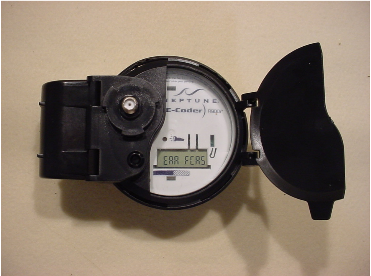
Figure 1: External – Top View (Display Cover Open)
