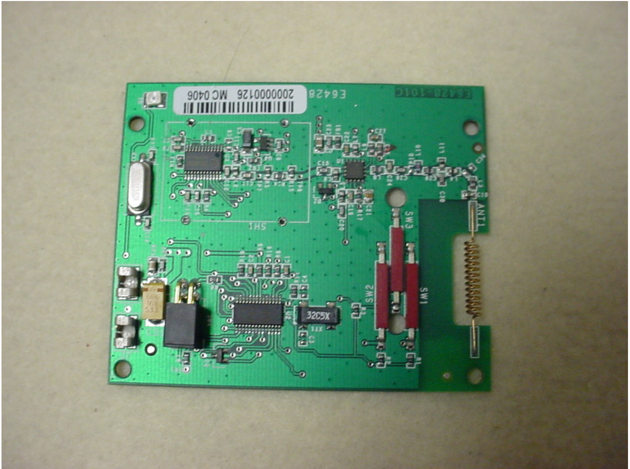
Figure 2: - Internal - PCB Top Unshielded
